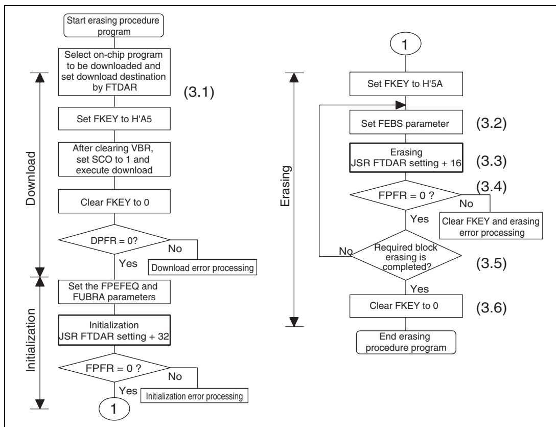
Figure 17.12 Erasing Procedure
