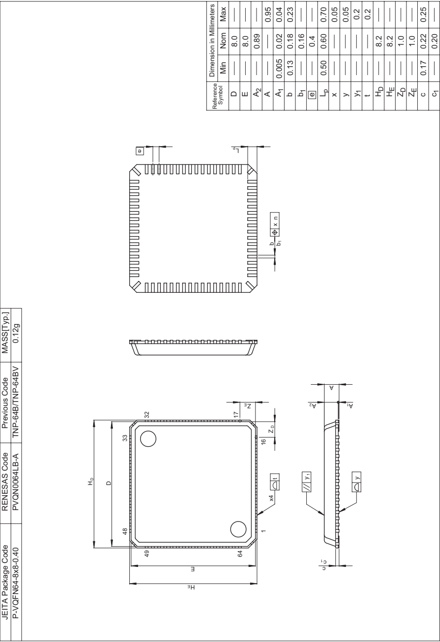
Figure C.4 VQFN-64
