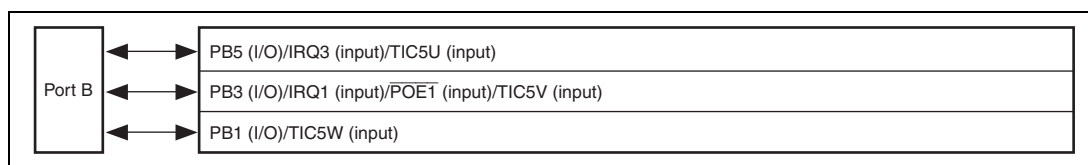
Figure 16.4 Port B (SH7124)
