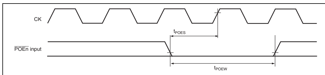
Figure 21.14 POE Input Timing
