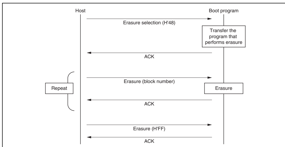
Figure 17.20 Sequence of Erasure
