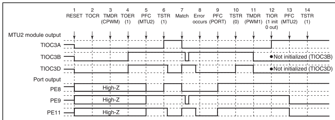
Figure 9.145 Error Occurrence in Complementary PWM Mode, Recovery in PWM Mode 1
