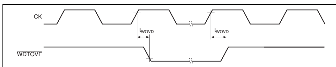
Figure 21.11 WDT Timing
