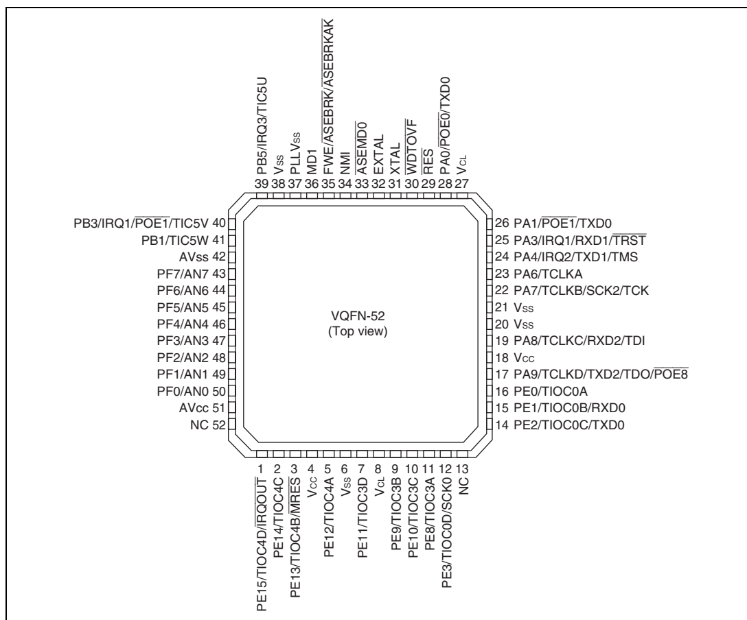
Figure 1.3 (2) Pin Assignments of SH7124
