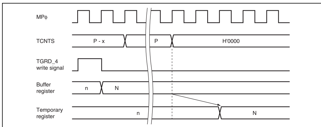
Figure 9.97 Transfer Timing from Buffer Register to Temporary Register (TCNTS Operating)
