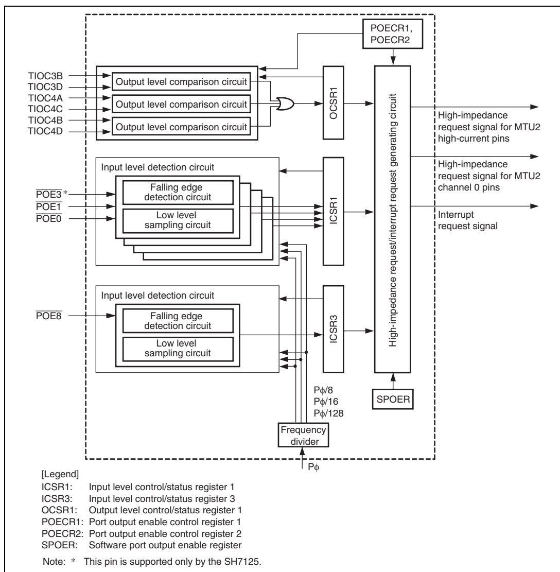
Figure 10.1 Block Diagram of POE
