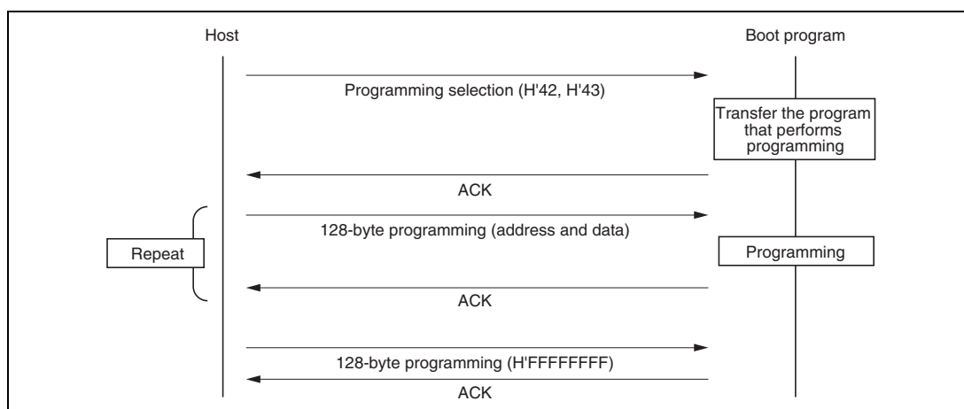
Figure 17.19 Sequence of Programming
