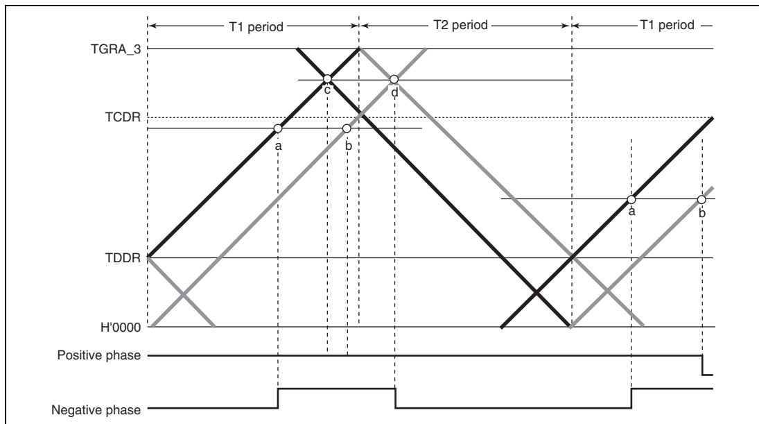
Figure 9.47 Example of Complementary PWM Mode Waveform Output (2)
