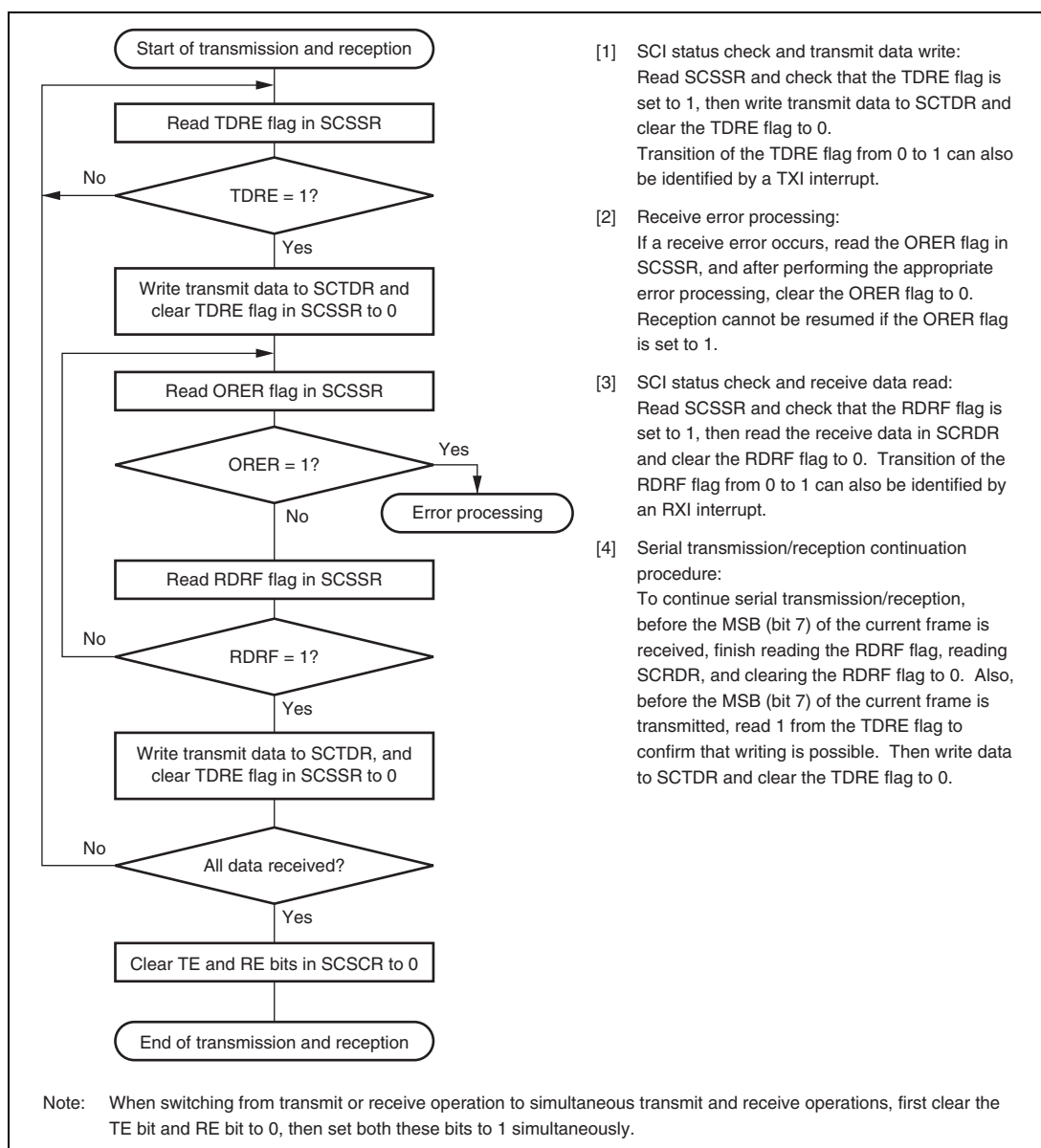
Figure 12.14 Sample Flowchart for Transmitting/Receiving Serial Data
