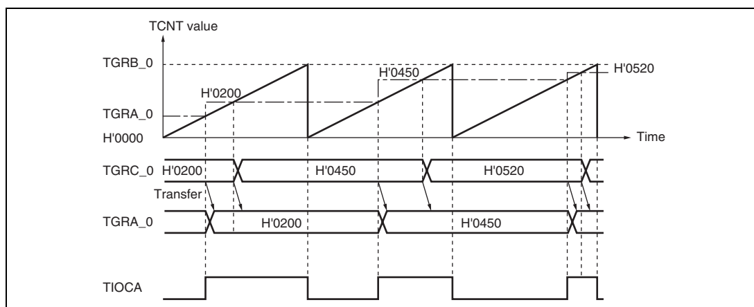
Figure 9.17 Example of Buffer Operation (1)
