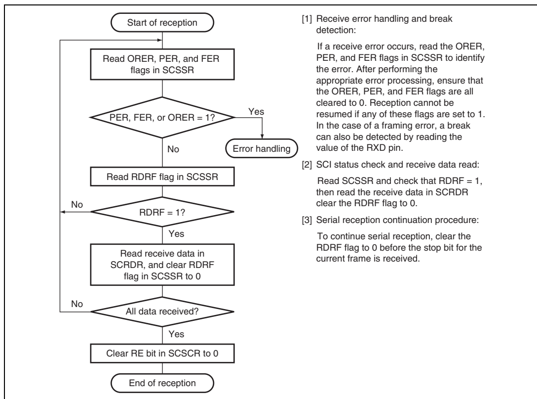
Figure 12.6 Sample Flowchart for Receiving Serial Data
