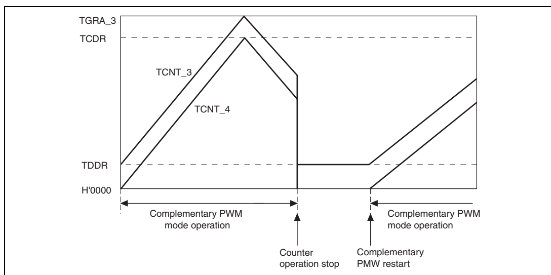
Figure 9.119 Counter Value during Complementary PWM Mode Stop
