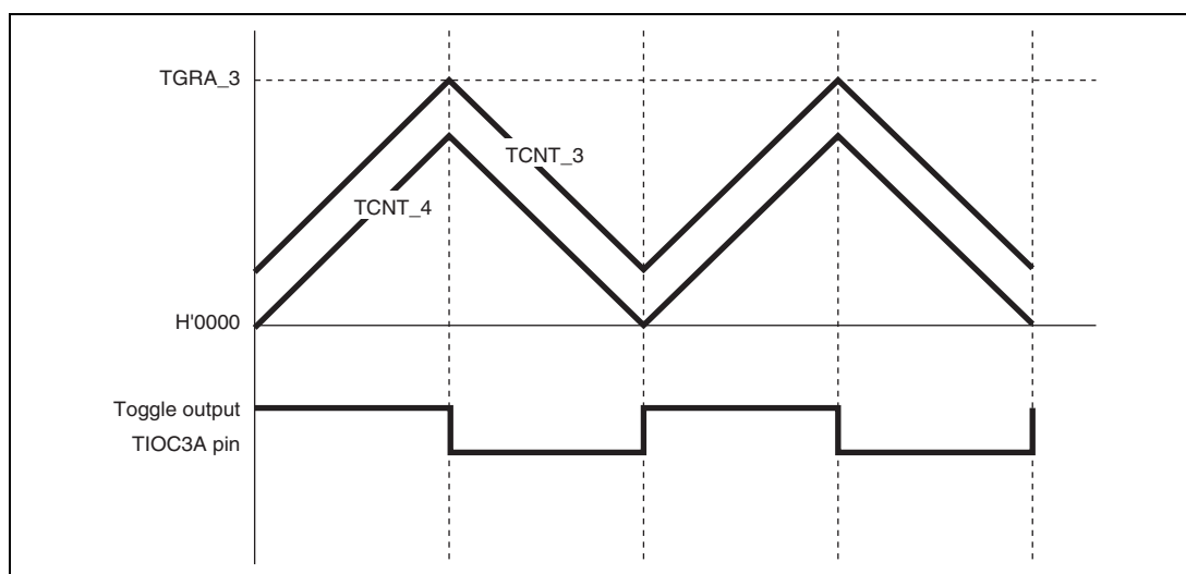
Figure 9.54 Example of Toggle Output Waveform Synchronized with PWM Output
