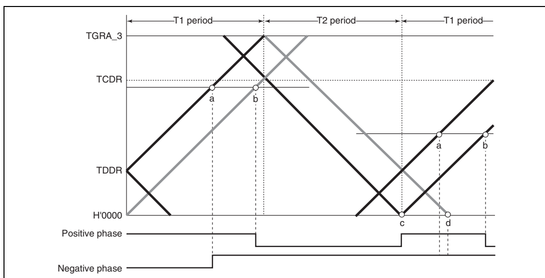
Figure 9.50 Example of Complementary PWM Mode 0% and 100% Waveform Output (2)
