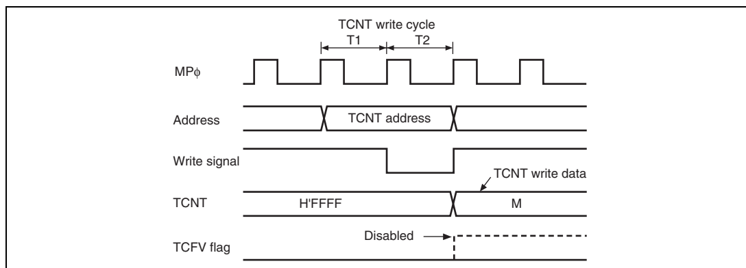
Figure 9.123 Contention between TCNT Write and Overflow
