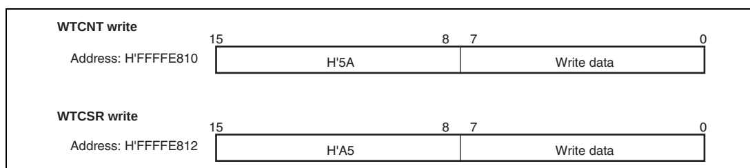
Figure 11.2 Writing to WTCNT and WTCSR
