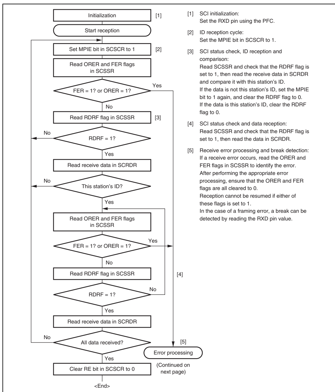
Figure 12.18 Sample Multiprocessor Serial Reception Flowchart (1)
