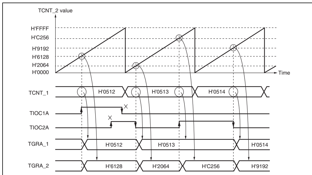
Figure 9.23 Cascaded Operation Example (c)
