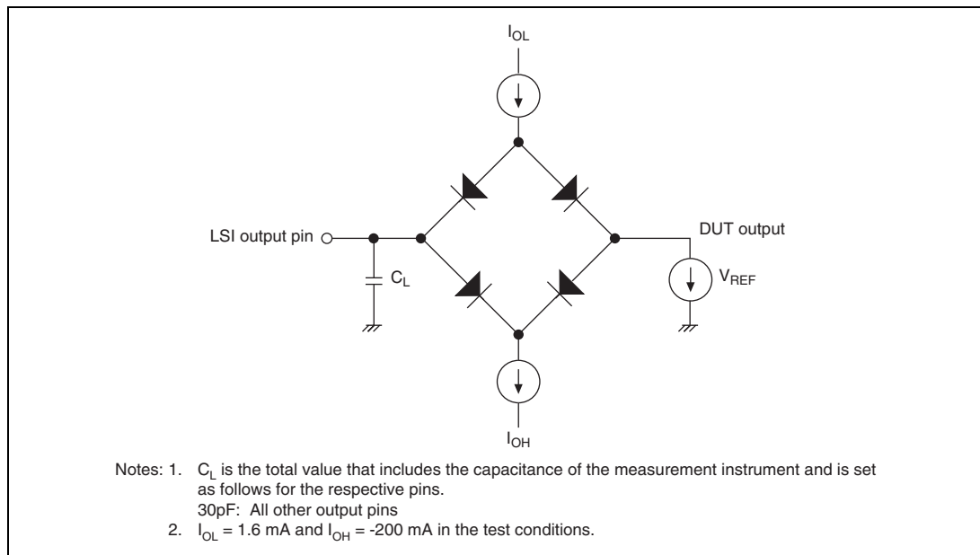
Figure 21.16 Output Load Circuit
