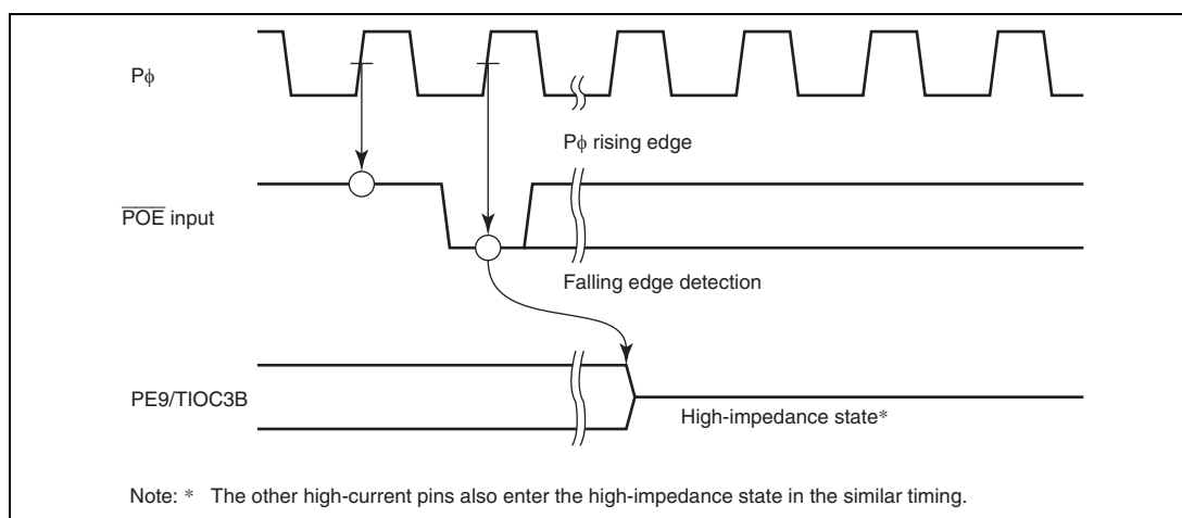
Figure 10.2 Falling Edge Detection
