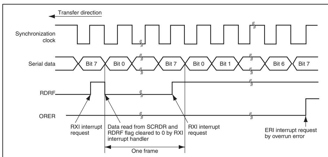
Figure 12.13 Example of SCI Receive Operation
