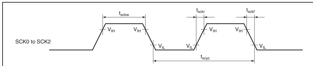
Figure 21.12 Input Clock Timing
