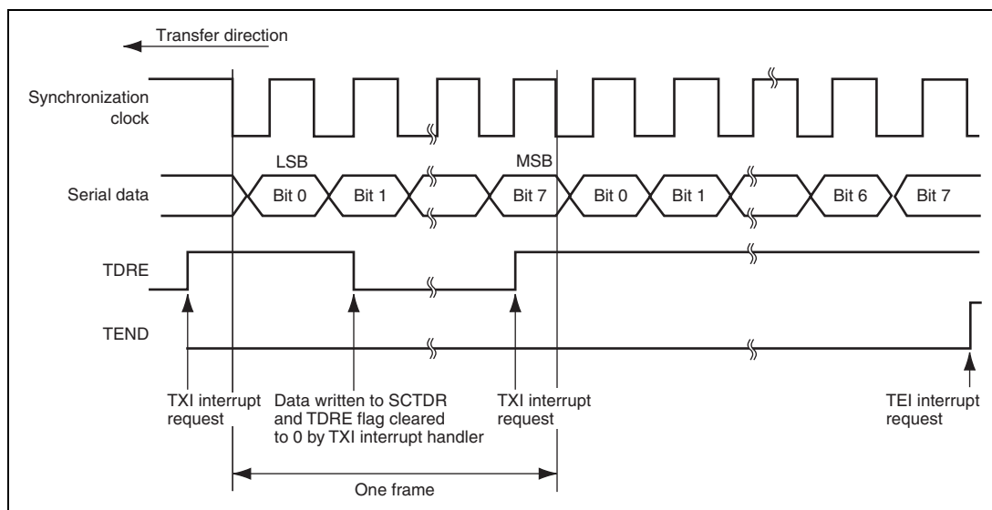
Figure 12.11 Example of SCI Transmit Operation
