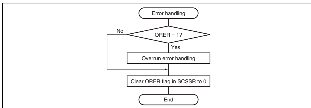
Figure 12.12 Sample Flowchart for Receiving Serial Data (2)
