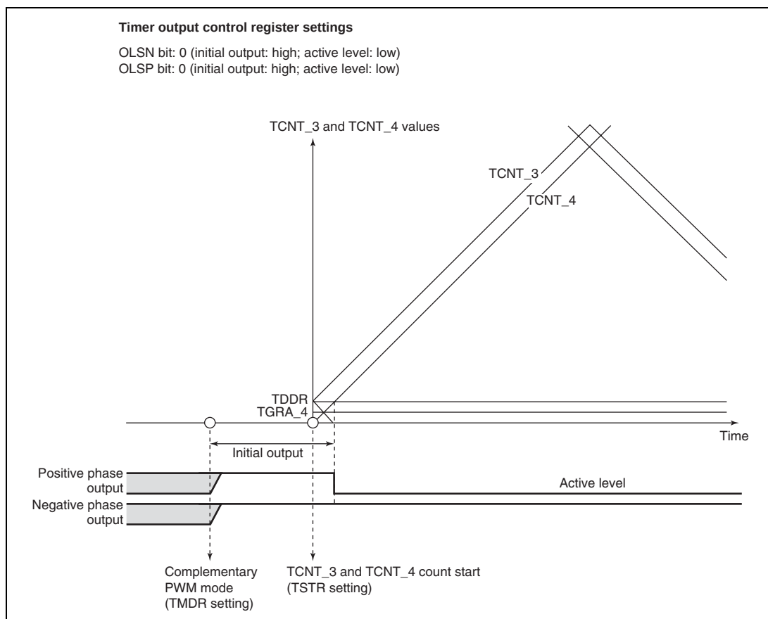
Figure 9.45 Example of Initial Output in Complementary PWM Mode (2)
