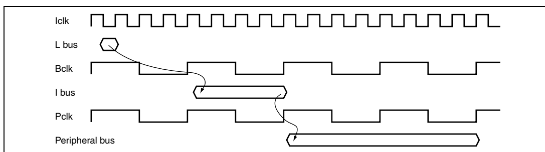
Figure 8.1 Timing of Write Access to the Peripheral Bus (Iclk:Bclk:Pclk = 4:1:1)
