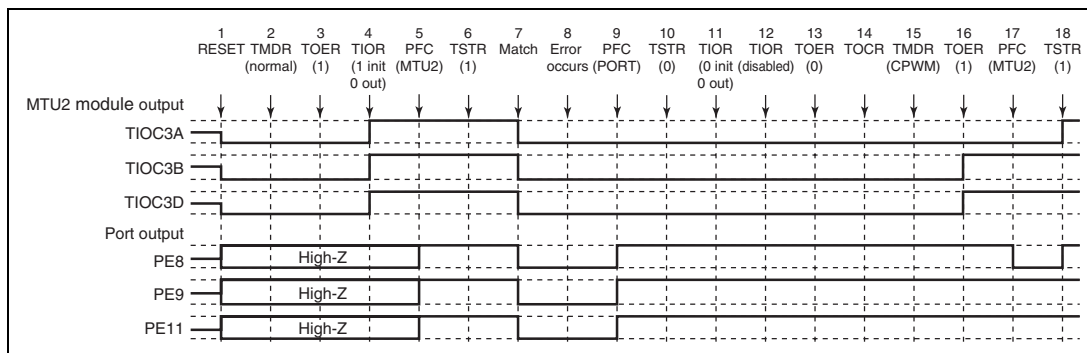
Figure 9.128 Error Occurrence in Normal Mode, Recovery in Complementary PWM Mode
