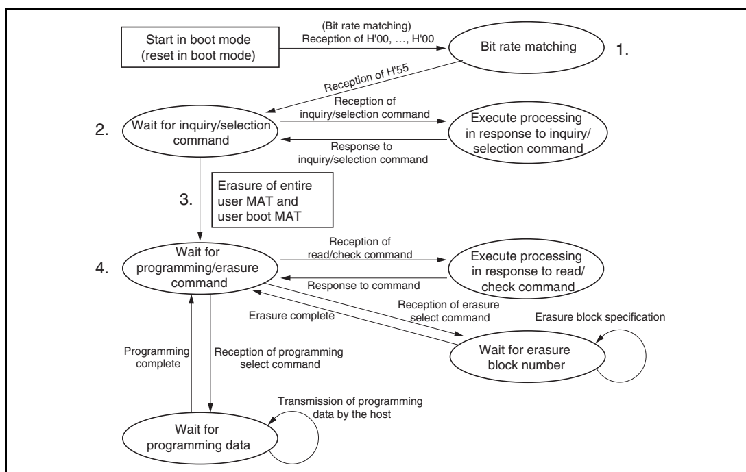
Figure 17.8 State Transitions in Boot Mode
