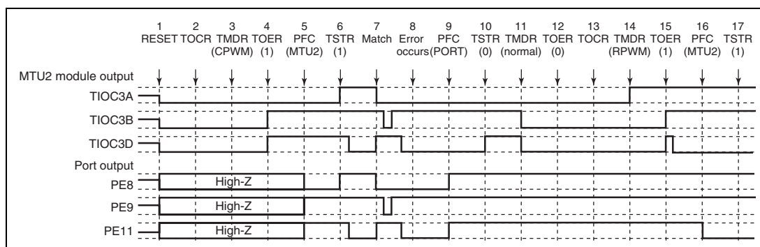
Figure 9.148 Error Occurrence in Complementary PWM Mode, Recovery in Reset-Synchronized PWM Mode
