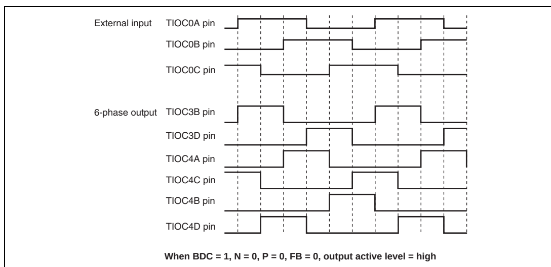
Figure 9.63 Example of Output Phase Switching by External Input (1)
