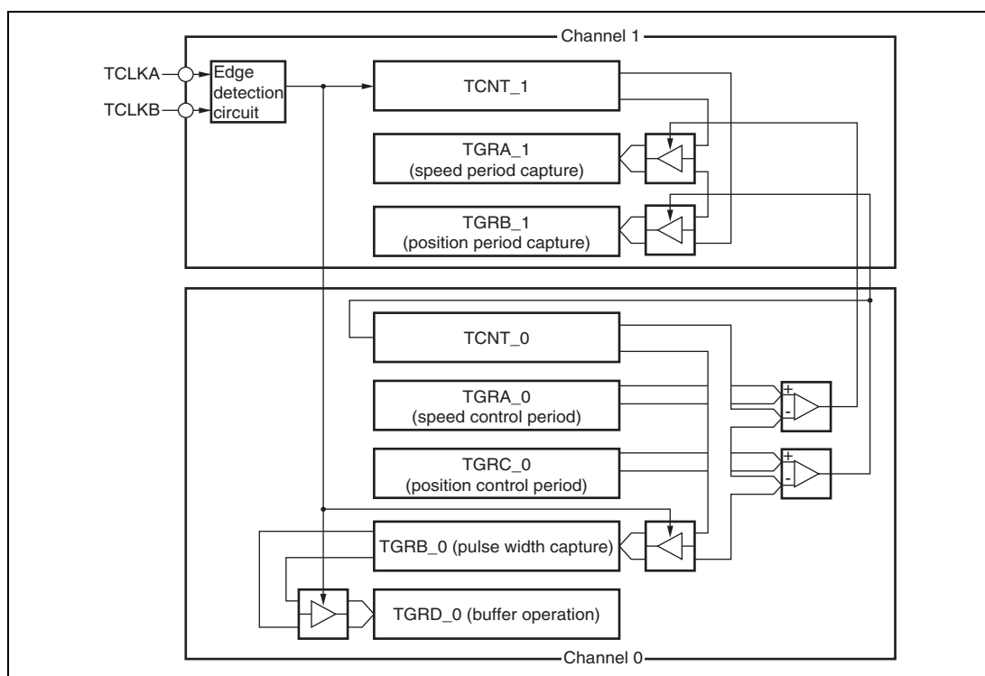
Figure 9.34 Phase Counting Mode Application Example
