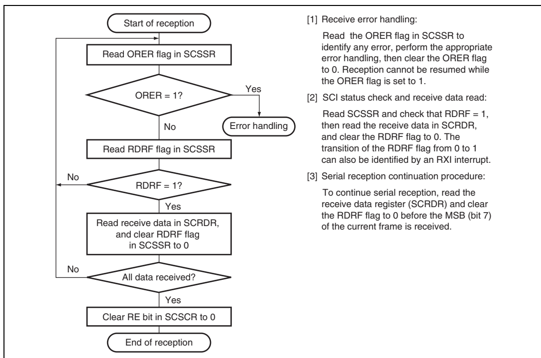
Figure 12.12 Sample Flowchart for Receiving Serial Data (1)
