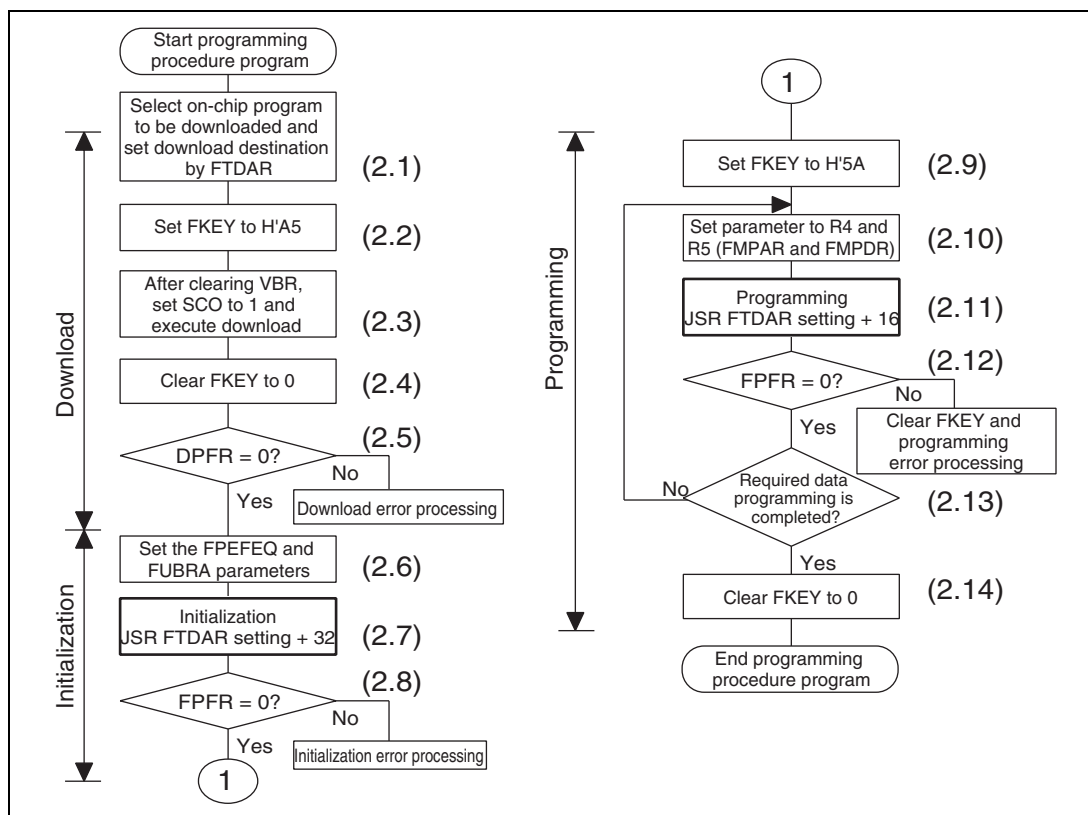
Figure 17.11 Programming Procedure
