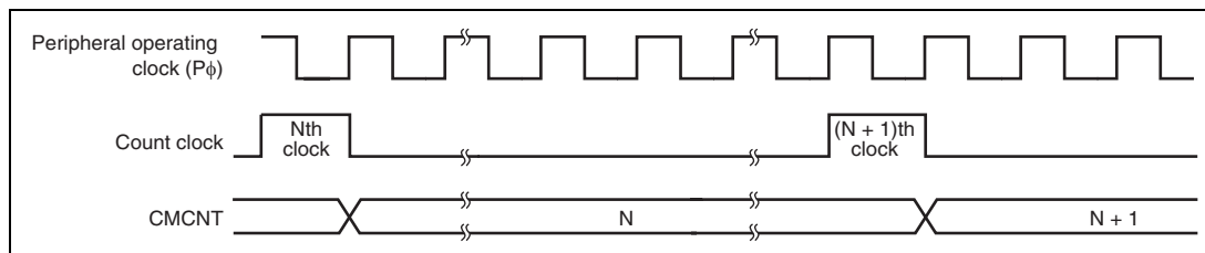
Figure 14.3 Count Timing
