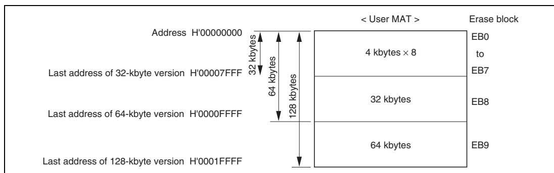
Figure 17.4 Block Division of User MAT
