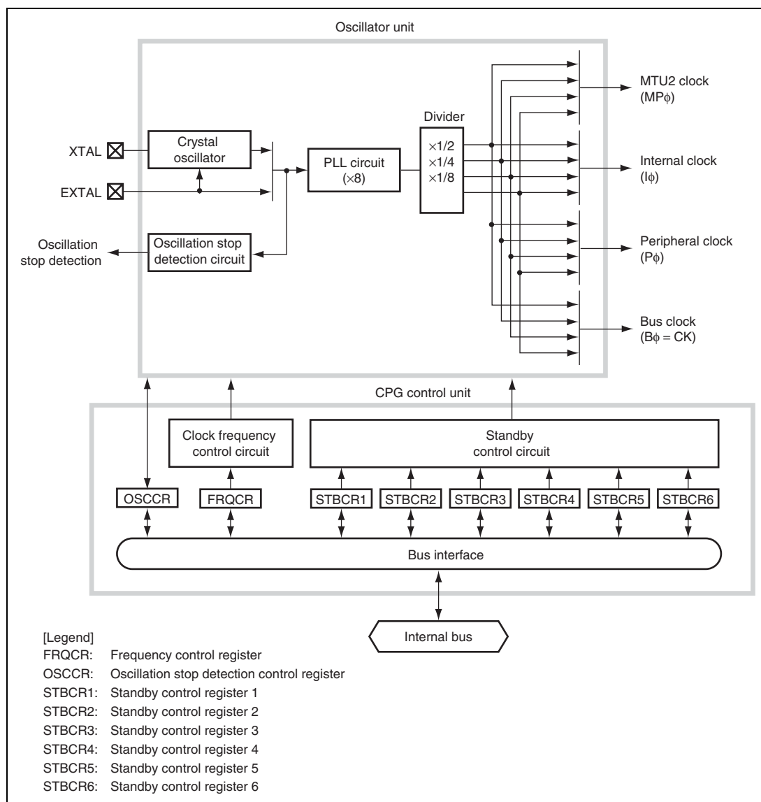
Figure 4.1 Block Diagram of CPG
