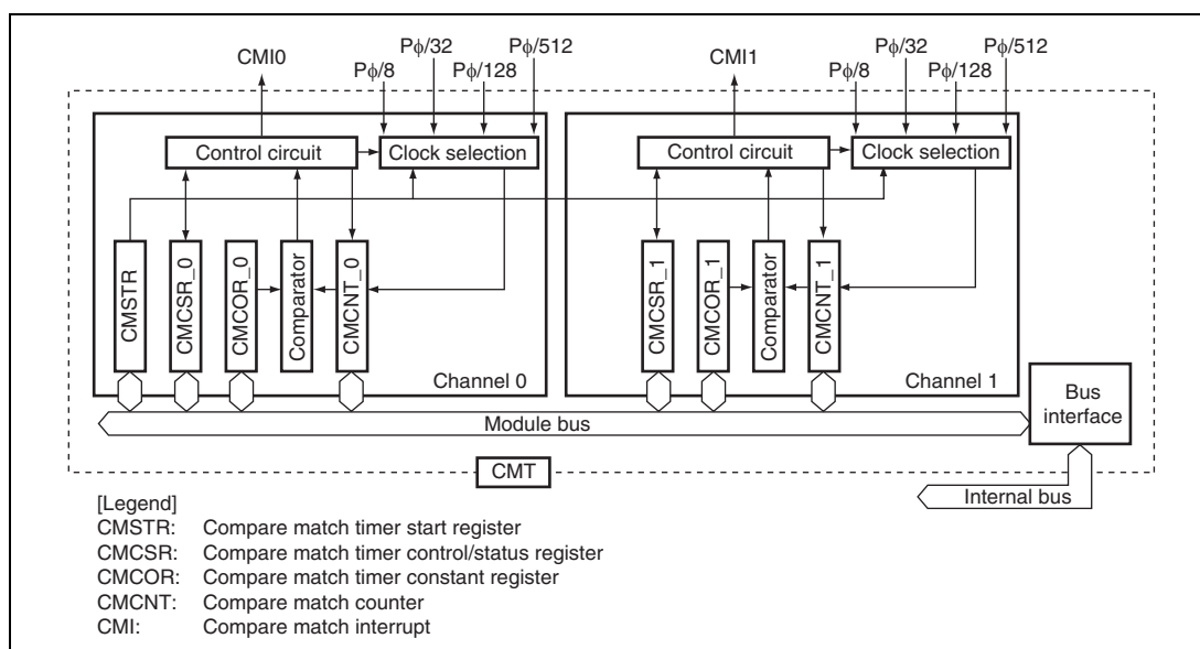
Figure 14.1 Block Diagram of CMT
