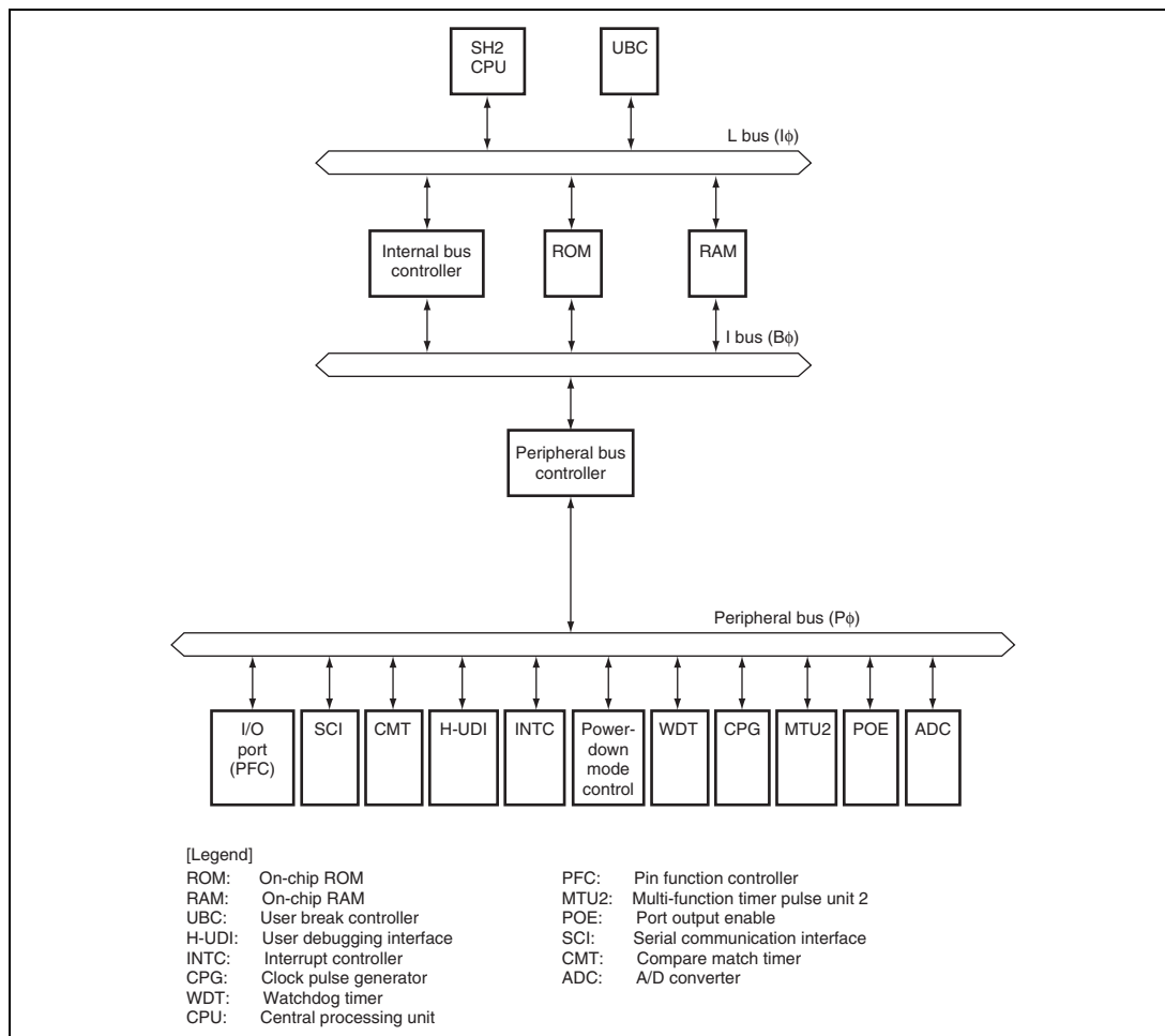
Figure 1.1 Block Diagram
