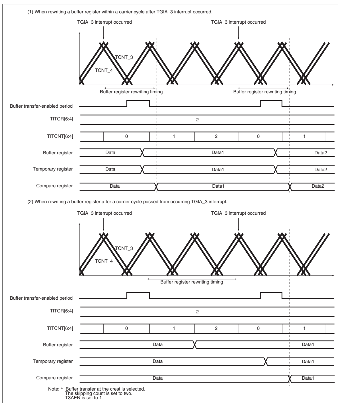
Figure 9.71 Example of Operation when Buffer Transfer is Linked with Interrupt Skipping (BTE1 = 1 and BTE0 = 0)
