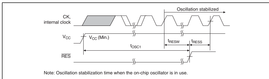
Figure 21.2 Power-On Oscillation Stabilization Time
