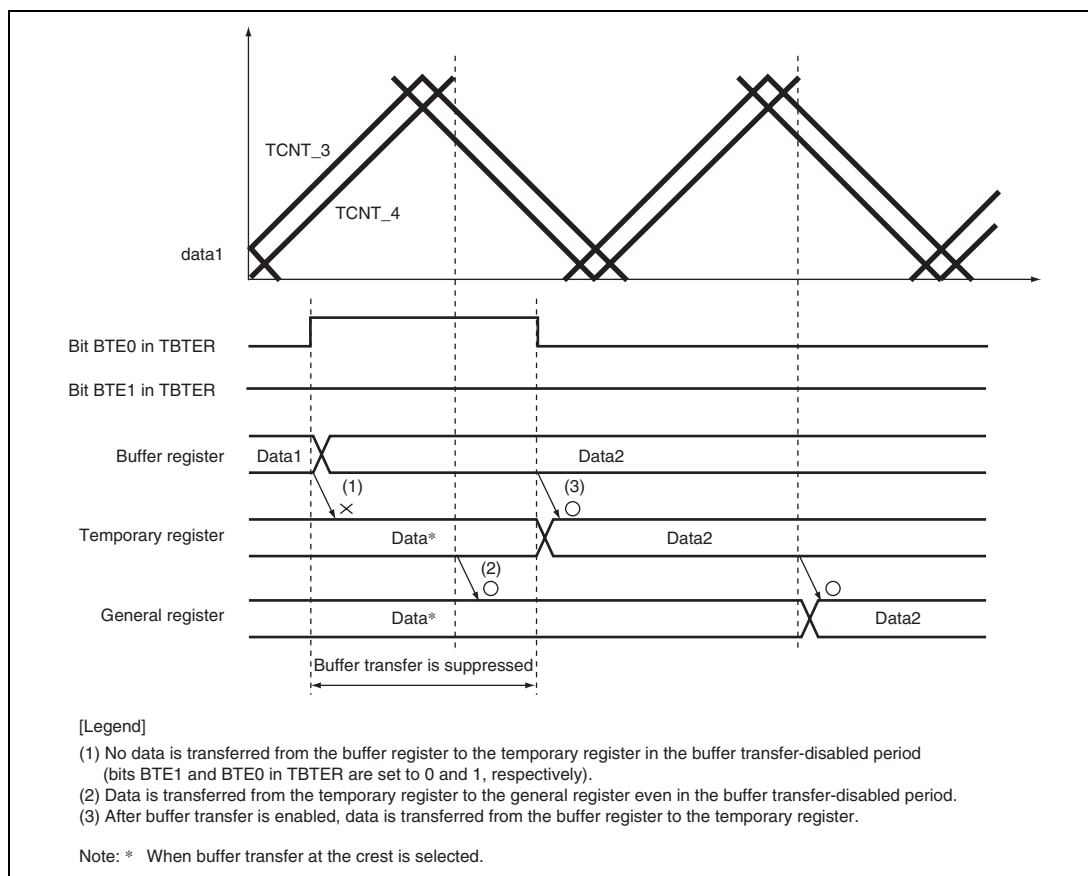
Figure 9.70 Example of Operation when Buffer Transfer is Suppressed (BTE1 = 0 and BTE0 = 1)
