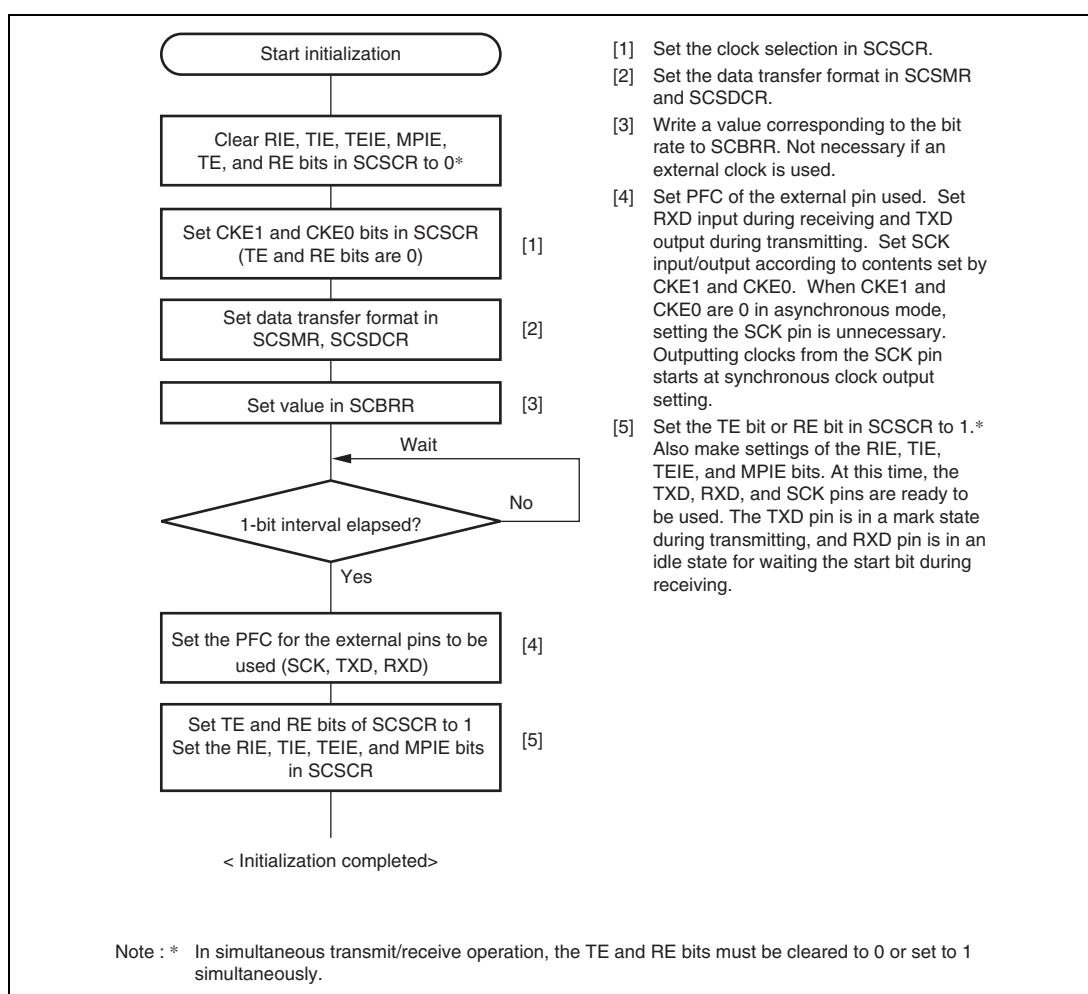
Figure 12.3 Sample Flowchart for SCI Initialization
