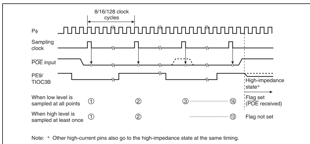
Figure 10.3 Low-Level Detection Operation
