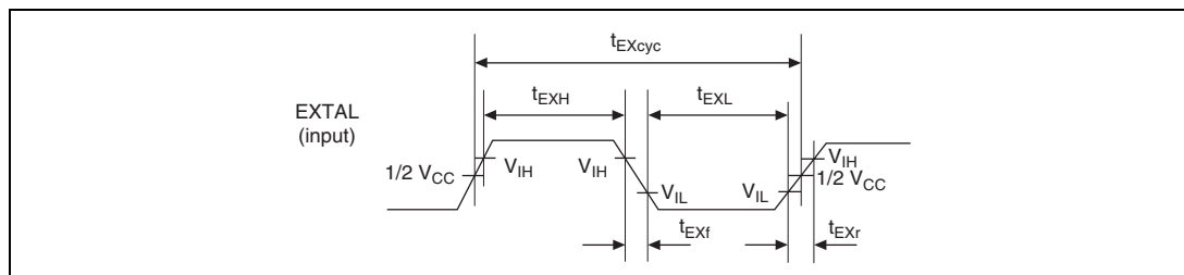
Figure 21.1 Timing of EXTAL Input Clock Signal
