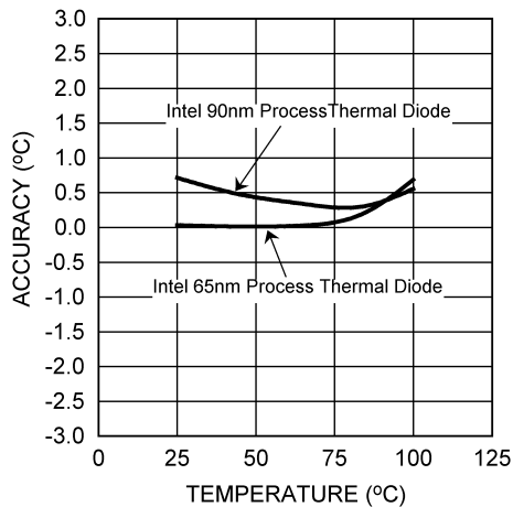
Thermal Diode Performance Comparison
