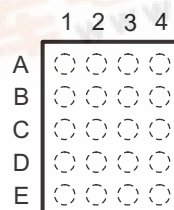
YFP PACKAGE (TOP VIEW)
