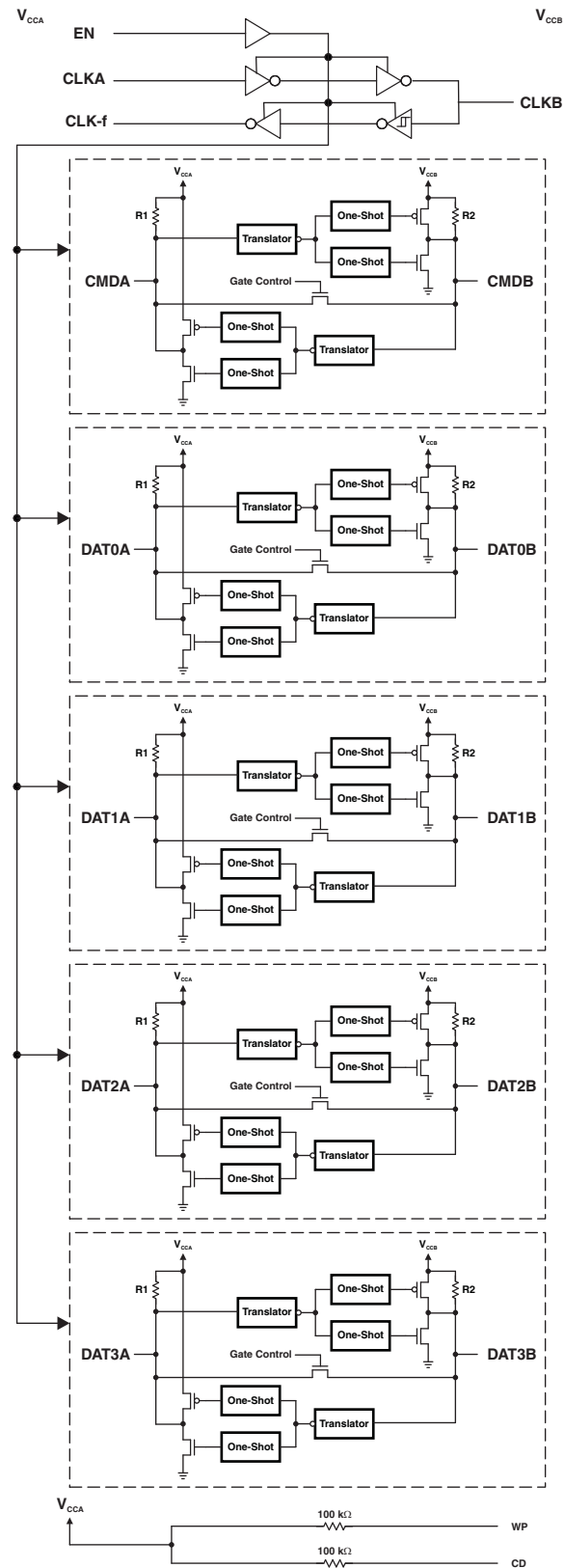
Figure 4. Logic Diagram
