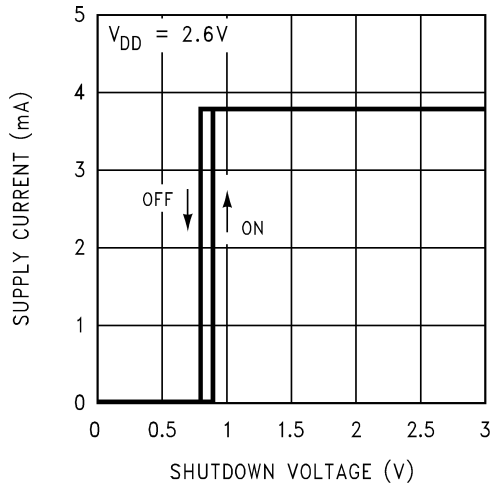
Shutdown Hysteresis Voltage
