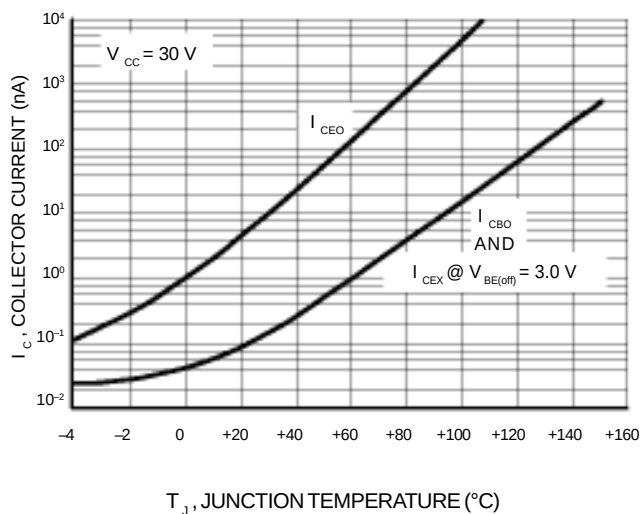
Figure 15. Typical Collector Leakage Current
