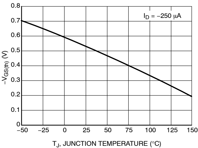
Figure 11. Threshold Voltage
