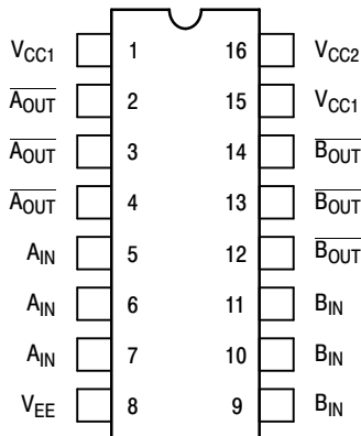
Figure 1. Logic Diagram
