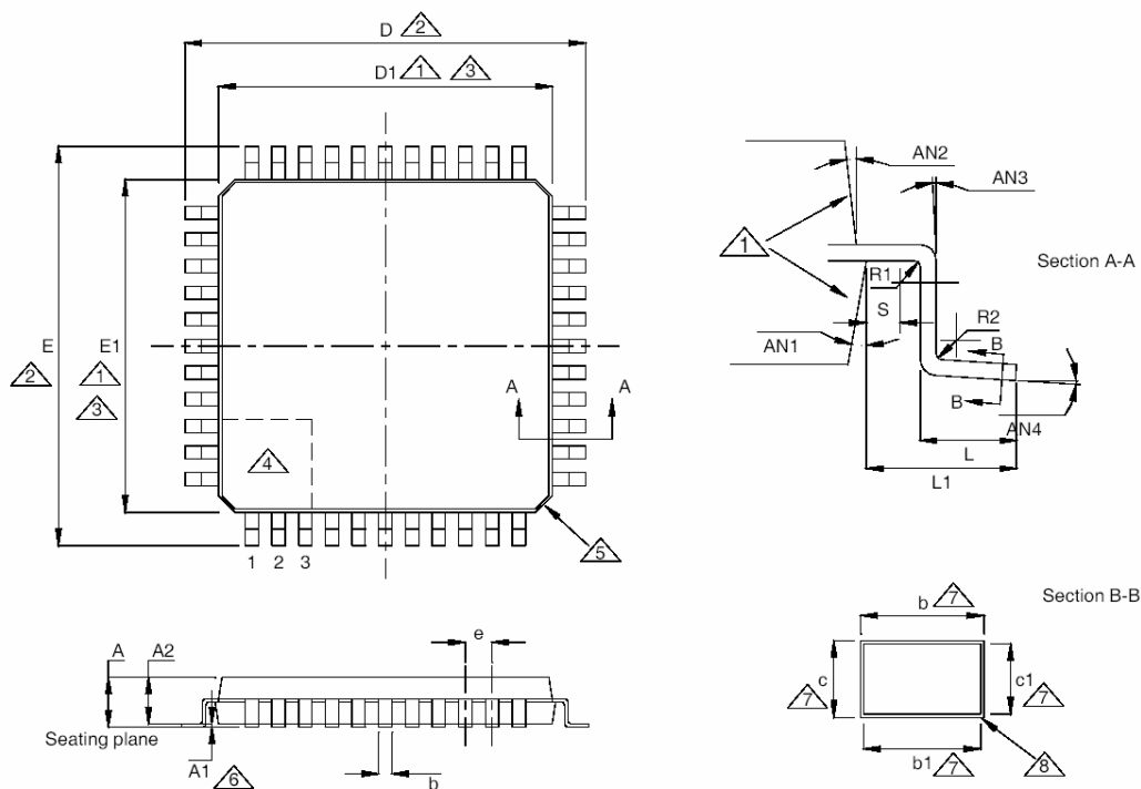
Figure 20 LQFP Package
