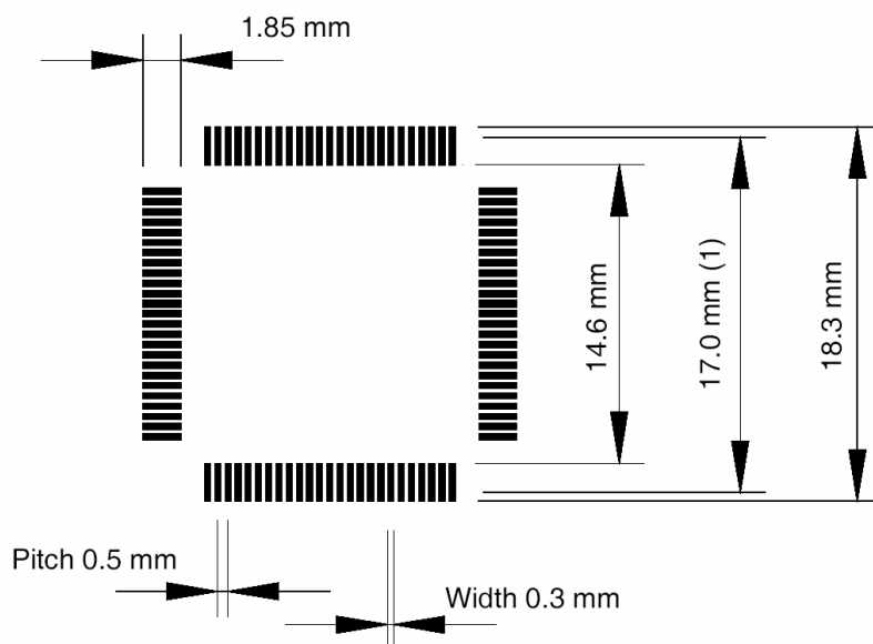
Figure 21 Typical 100 Pin LQFP Footprint
