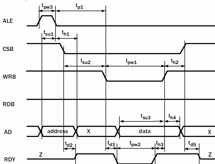
Figure 10 Write Access Timing in MULTIPLEXED Mode
