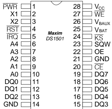
DIP, SO
