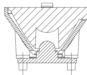
Section through 4° LED Optic, Optic Holder and Luxeon 1W star board
