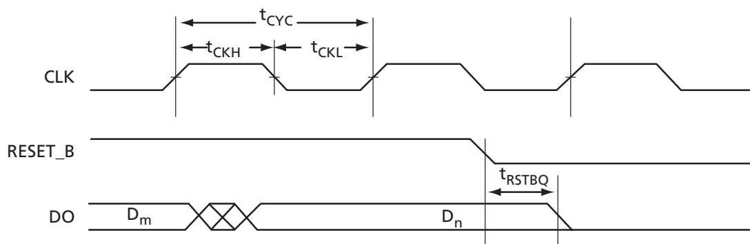
Figure 2-57 • RAM Reset
