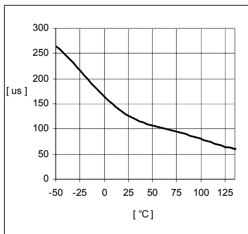
Propagation Time t_p vs. Temperature
