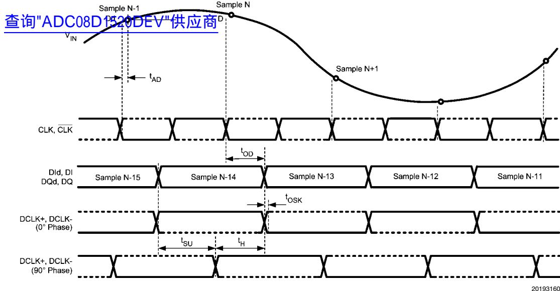
FIGURE 5. DDR Clocking in Non-Demultiplexed Non-DES Mode
