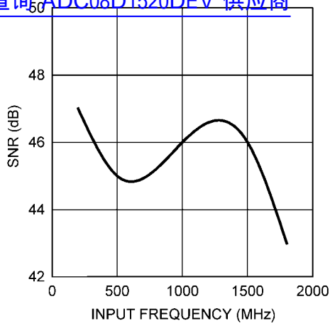
SNR vs. INPUT FREQUENCY 查询"ADC08D1520DEV"供应商
