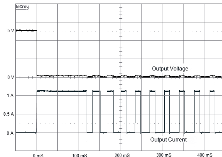
Figure 2. Current Over load Condition. Load Switch turned on with 0.1 Ω load at time = 0 ms.
