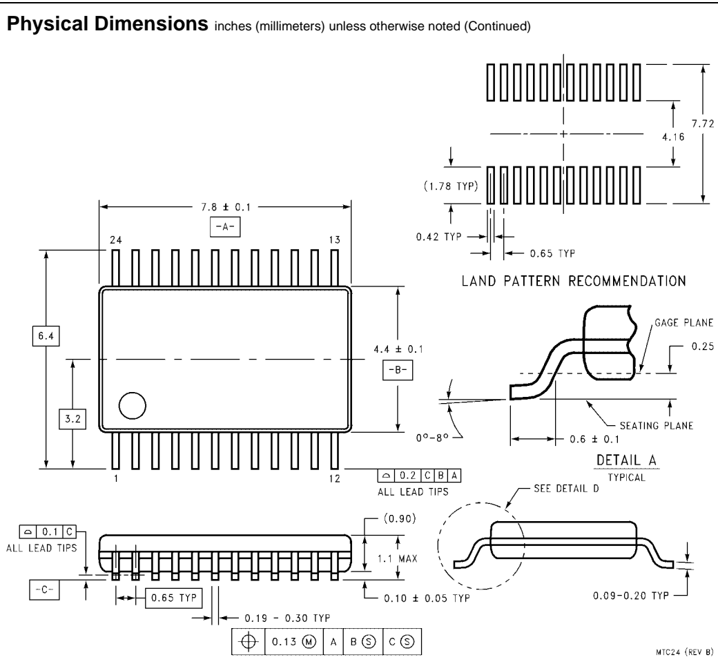
20-Lead Thin Shrink Small Outline Package (TSSOP), JEDEC MO-153, 4.4mm Wide Package Number MTC24
