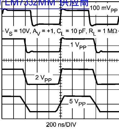
Step Response for Various Amplitudes 查询"LM7332MM"供应商
