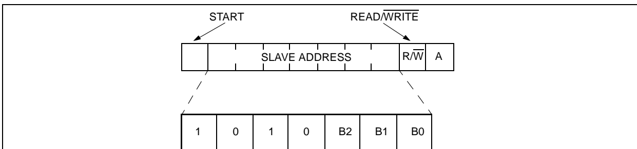
FIGURE 3-4: CONTROL BYTE ALLOCATION
