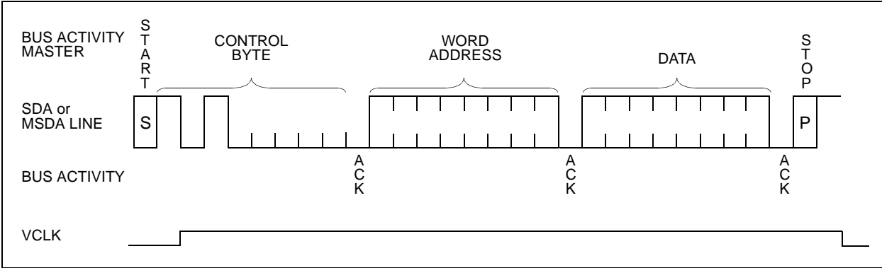
FIGURE 4-1: BYTE WRITE
