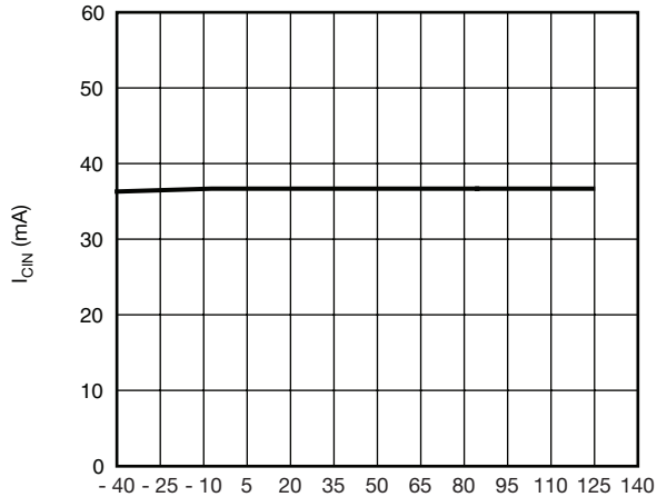
Temperature (°C) ICIN + IDRIV (mA) vs. Temperature at Frequency = 1 MHz D = 10 \%, V_{CIN} = V_{DRV} = 5 V
