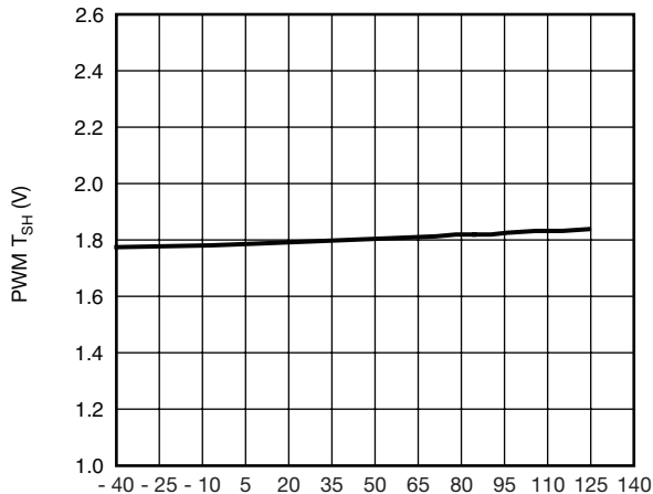
Temperature (°C) PWM Falling Tristate (V) vs. Temperature (°C) V_{CIN} = V_{DRV} = 5 V
