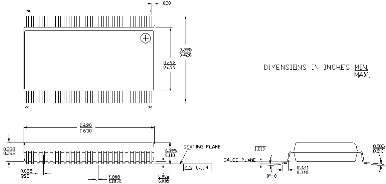
Figure 19. 48-Pin SSOP (51-85061)
