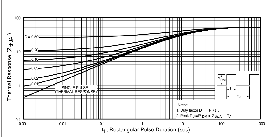
Figure 13. Maximum Effective Transient Thermal Impedance, Junction-to-Ambient
