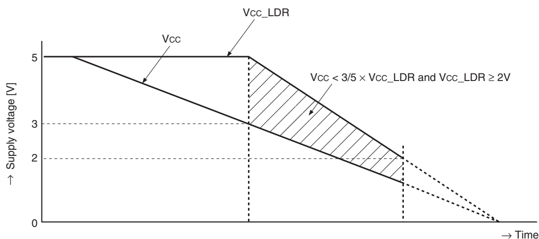
Fig. 1. Vcc and Vcc_LDR Power-off
