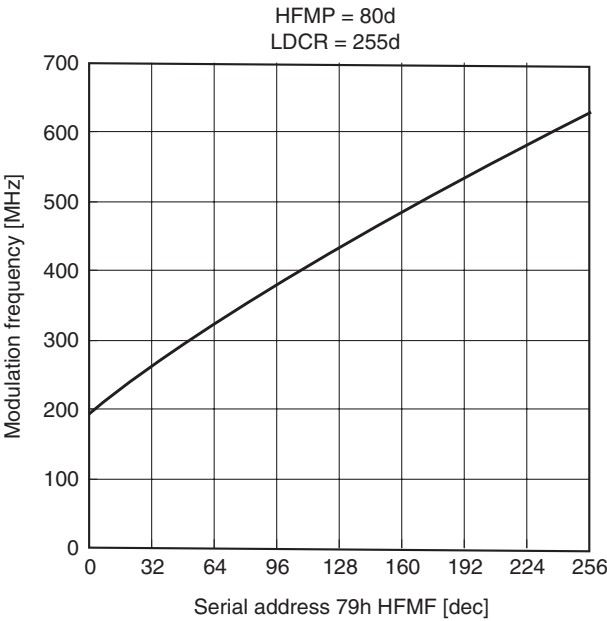
Control characteristics of HFMF and modulation frequency
