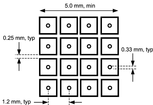
FIGURE 18. Recommended Package Land Pattern
