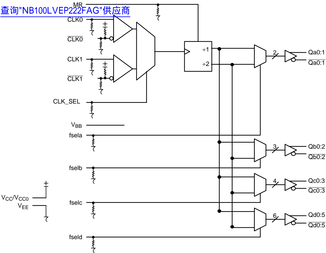
Figure 2. Logic Diagram
