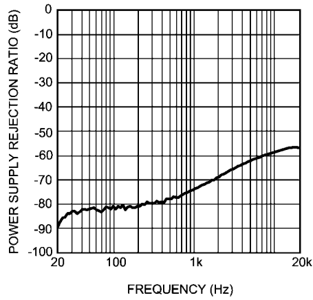
PSRR vs Frequency 查询"LM48820"供应商 V_{DD} = 3V, R_L = 16\Omega
