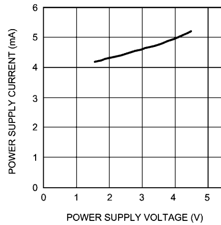
Power Supply Current vs Power Supply Voltage V_{IN} = 0V, \text{Stereo}
