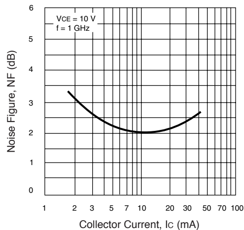
NE85635 NOISE FIGURE vs. COLLECTOR CURRENT
