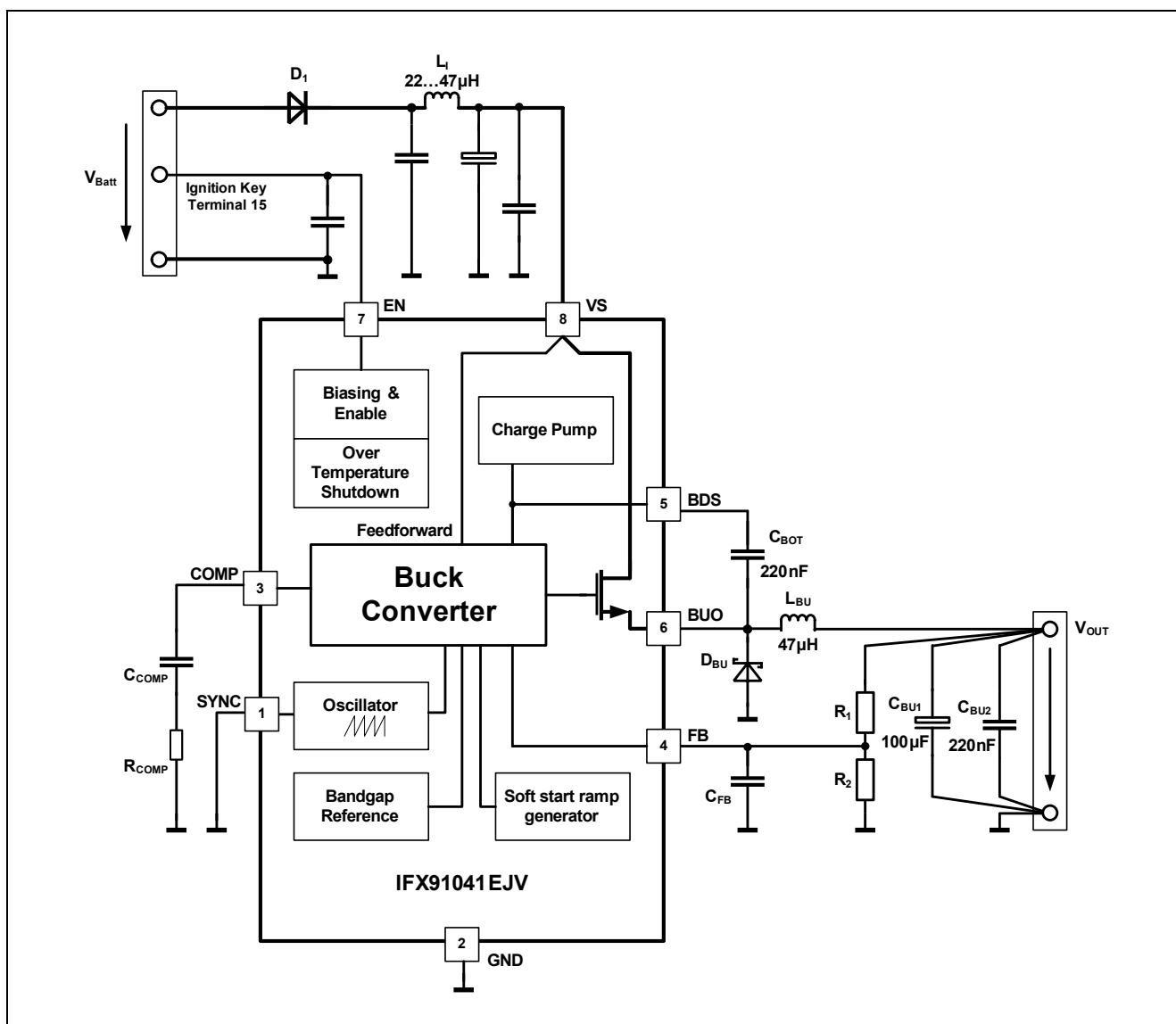
Figure 6 Application Diagram IFX91041EJV
