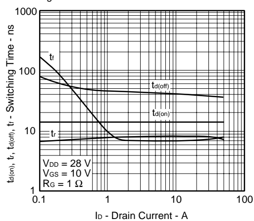
Figure15. SWITCHING CHARACTERISTICS
