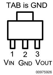
Top View LM2936MP
