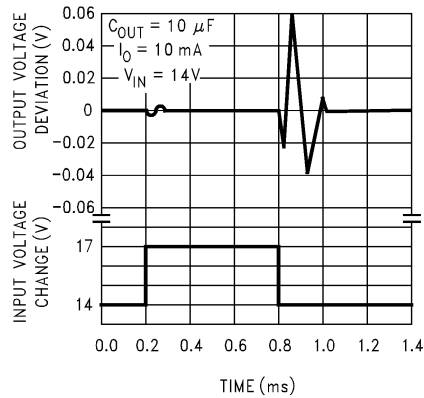
LM2936-5.0 Line Transient Response
