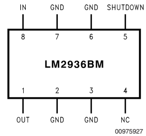
Top View LM2936BM and LM2936HVBMA See NS Package Number M08A
