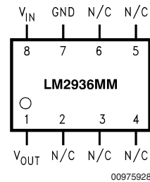
Top View LM2936MM See NS Package Number MUA08A
