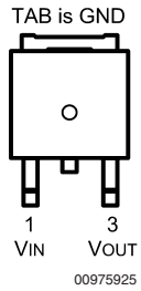
Top View LM2936DT
