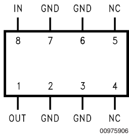
Top View LM2936M and LM2936HVMA See NS Package Number M08A
