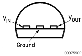
Bottom View LM2936Z See NS Package Number Z03A
