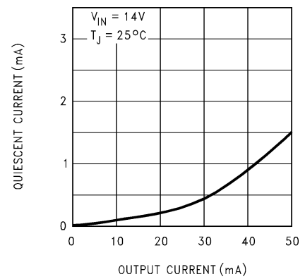
Quiescent Current
