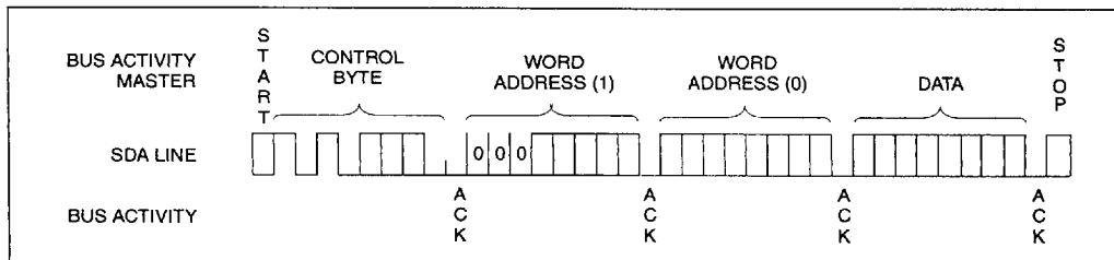
FIGURE 4-1: BYTE WRITE
