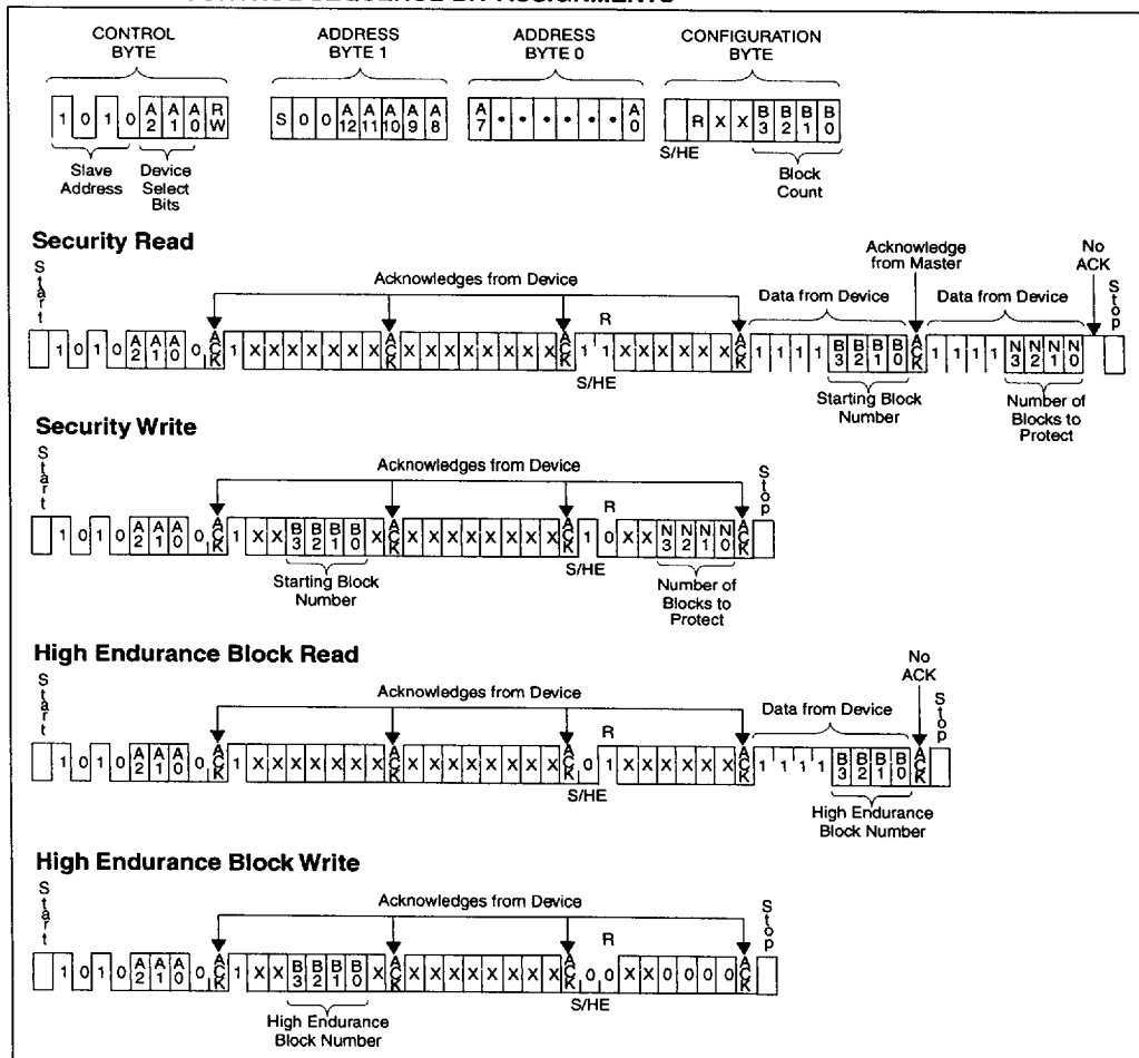
FIGURE 8-1: CONTROL SEQUENCE BIT ASSIGNMENTS
