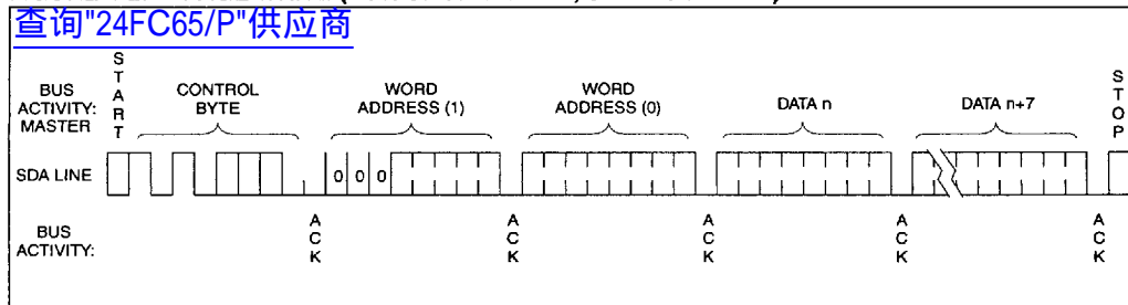
FIGURE 4-3: CURRENT ADDRESS READ
