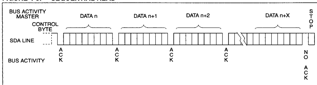
FIGURE 4-5: SEQUENTIAL READ
