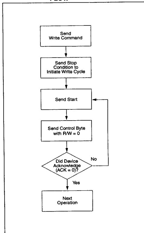
FIGURE 6-1: ACKNOWLEDGE POLLING FLOW
