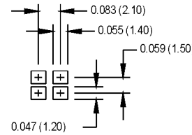
SUGGESTED SOLDER PAD LAYOUT
