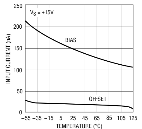
Input Currents
