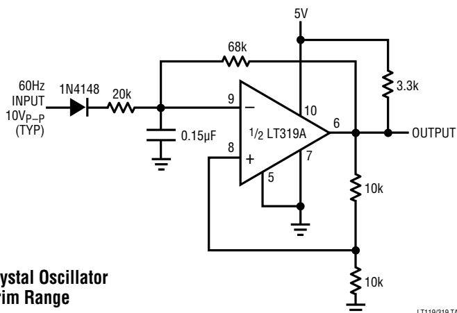
High Noise Immunity 60Hz Sync Circuit
