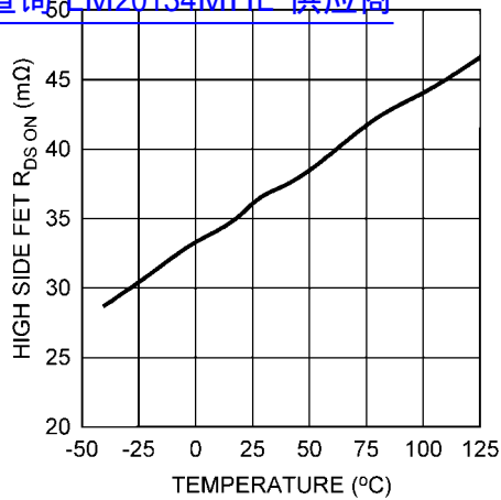
High-Side FET resistance vs. Temperature 查询"LM20134MHE"供应商
