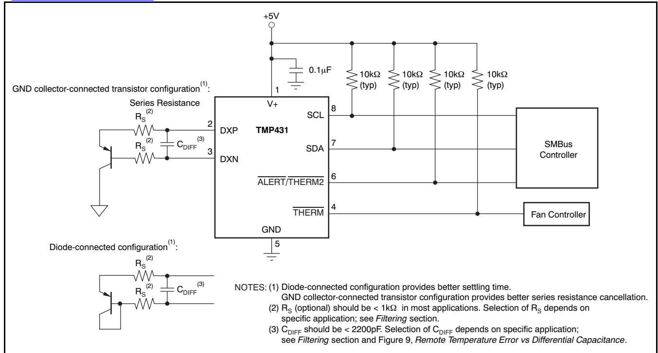
Figure 13. TMP431 Basic Connections
