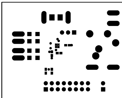
FIGURE 9. Solder Mask
