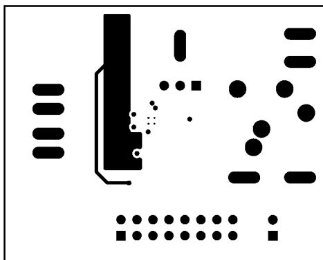
FIGURE 13. Layer 3 ( V_{DD} )
