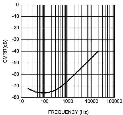
CMRR vs Frequency V_{DD} = 3.6\text{V} , V_{CM} = 1\text{V}_{P-P} , R_L = 32\Omega
