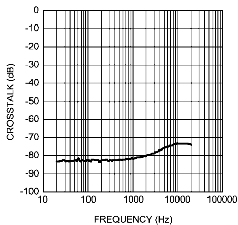
Crosstalk vs Frequency V_{DD} = 3.6\text{V} , V_{RIPPLE} = 1\text{V}_{P-P} , R_L = 32\Omega
