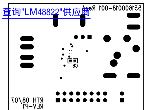
FIGURE 15. Bottom Silkscreen
