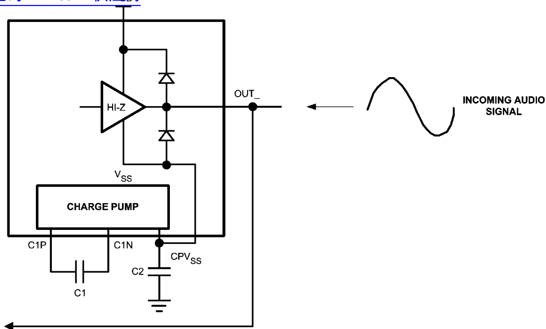
FIGURE 5. Back-Driving the LM48822 Outputs
