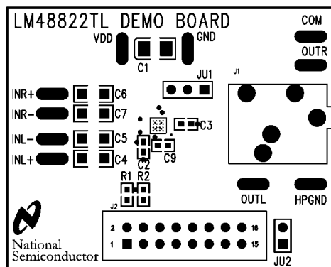
FIGURE 10. Top Silkscreen
