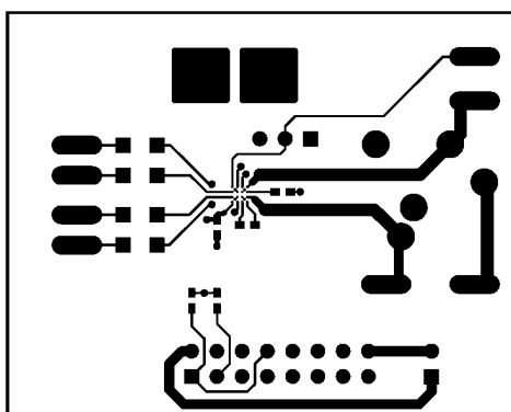
FIGURE 11. Top Layer
