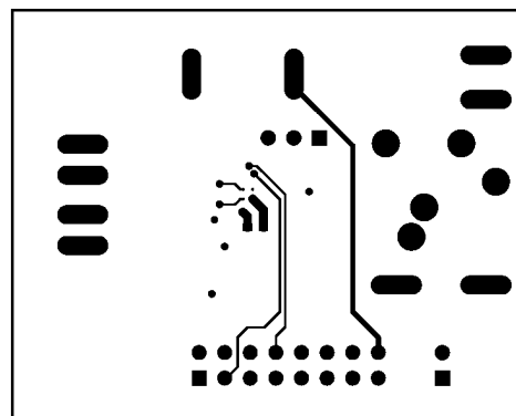
FIGURE 14. Bottom Layer
