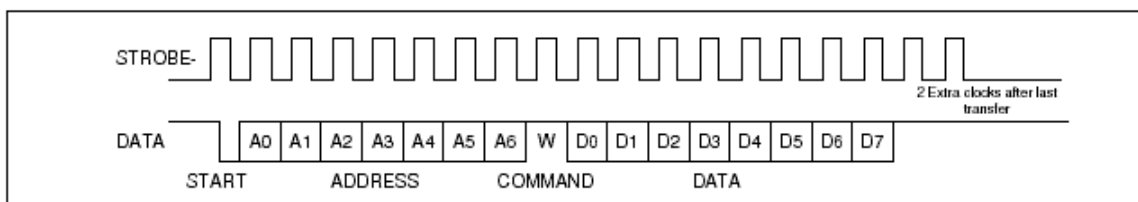
Figure 4 - Write Command
