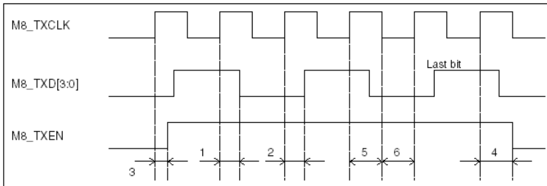
Figure 7 - Transmit Timing
