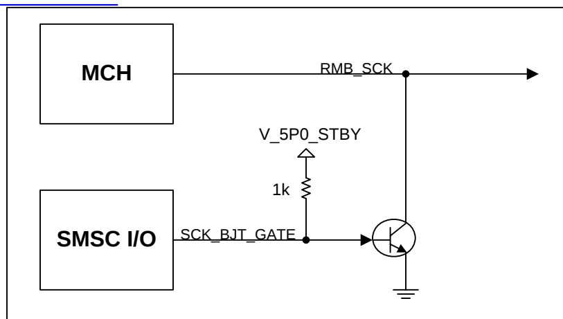
Figure 7.15 - SCK_BJT_Gate Circuit
