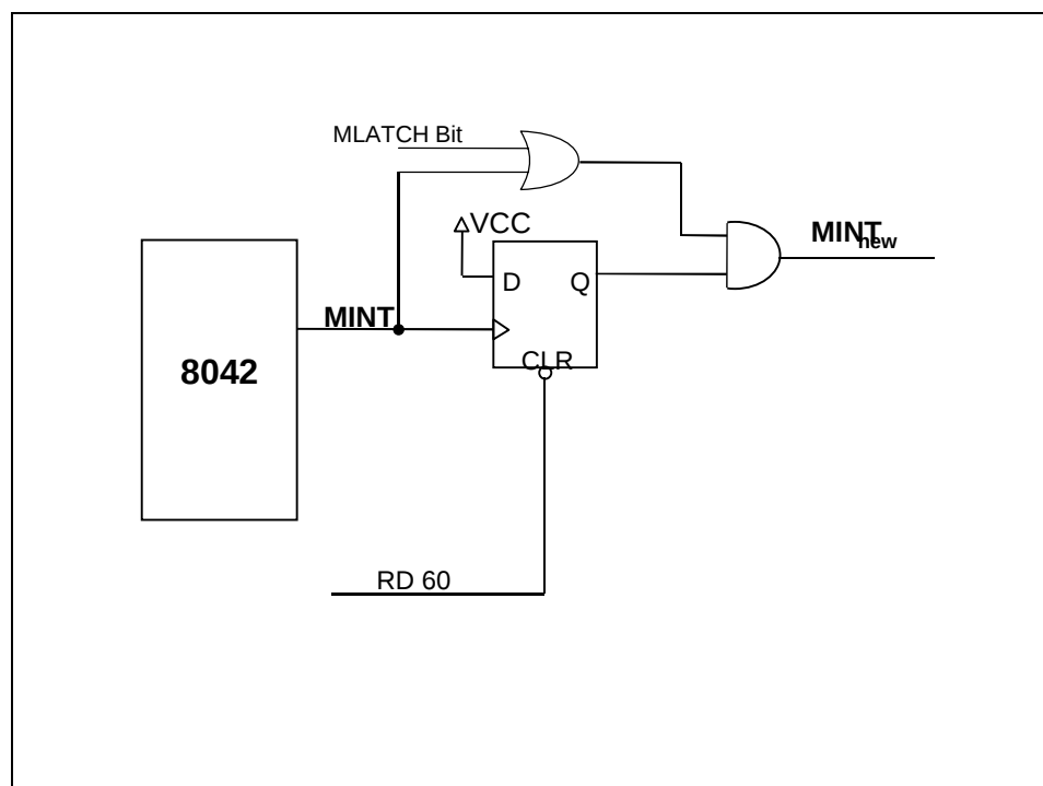
Figure 7.3 - Mouse Latch
