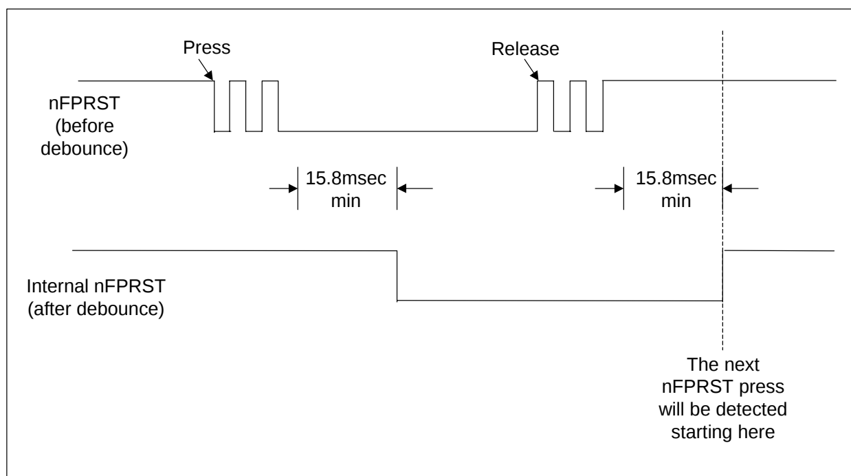
Figure 7.14 - NFPRST Timing
