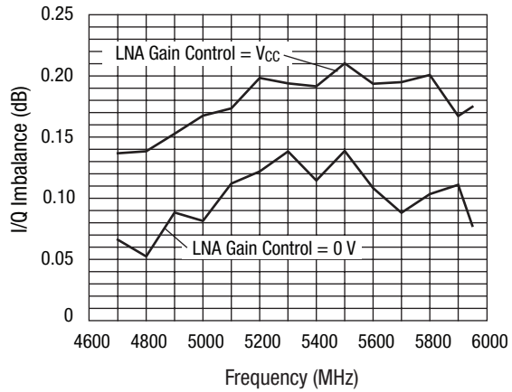
I/Q Imbalance vs. Frequency
