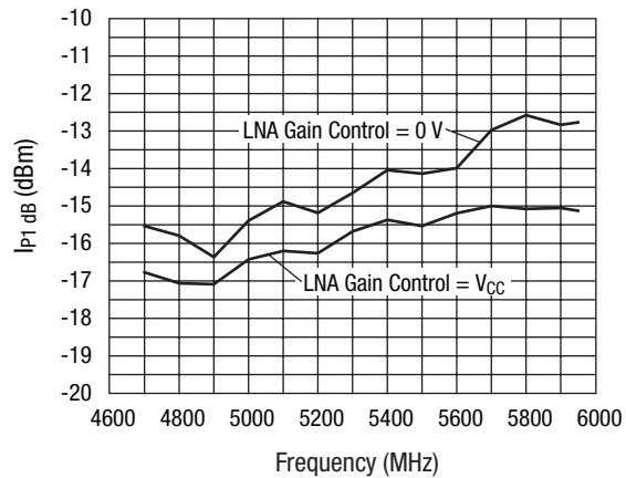
Input 1 dB Compression Point vs. Frequency
