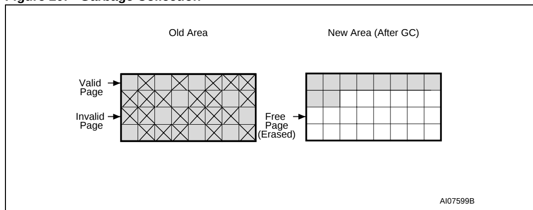
Figure 20. Garbage Collection
