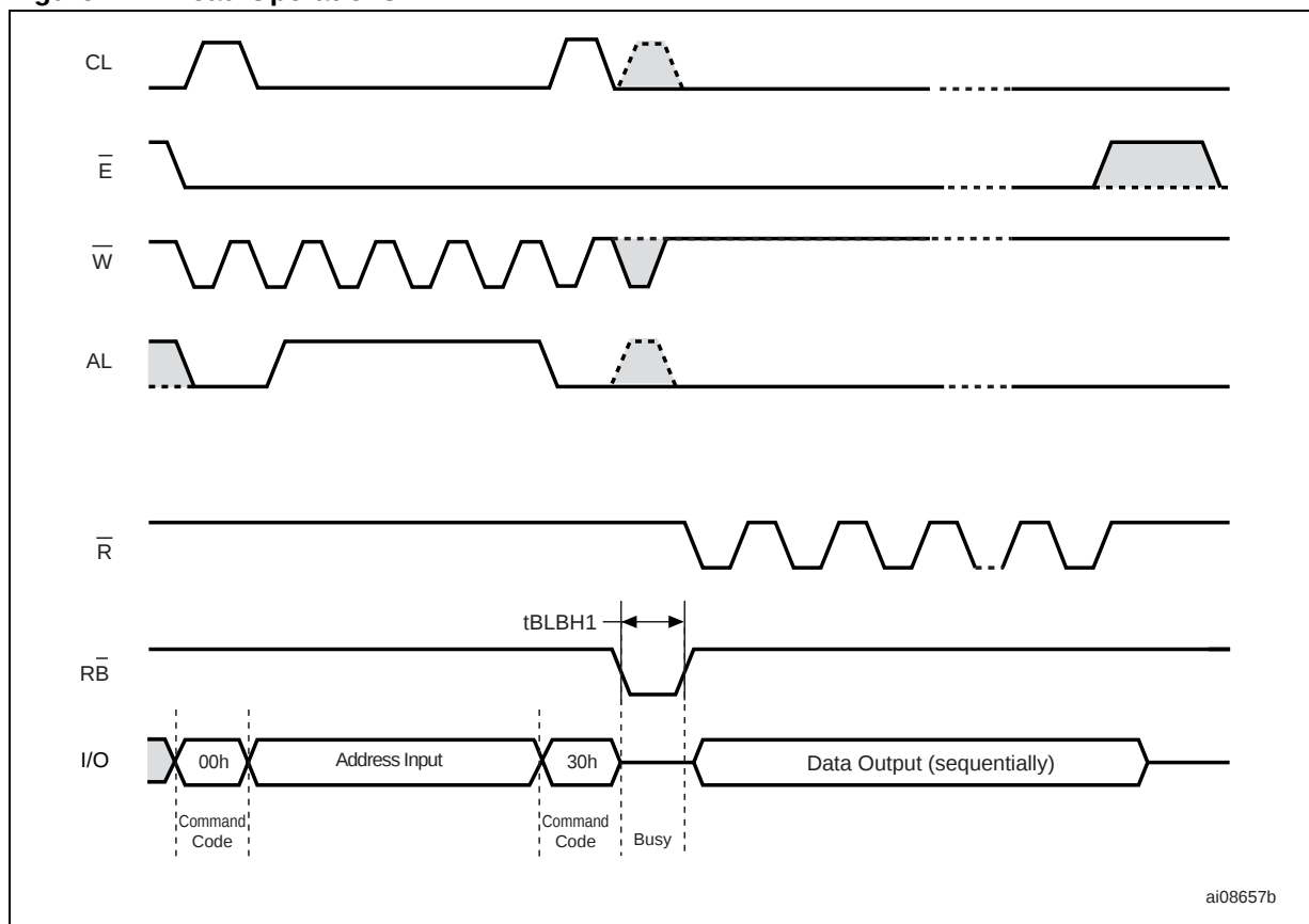
Figure 7. Read Operations
