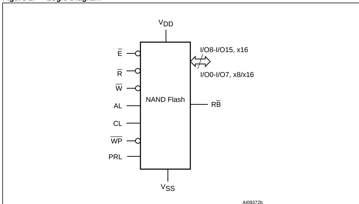
Figure 2. Logic Diagram
