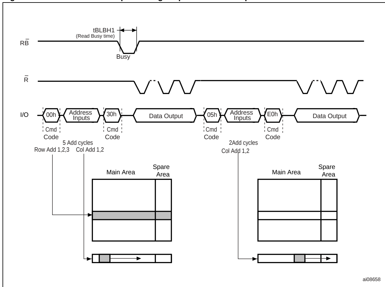
Figure 8. Random Data Output During Sequential Data Output
