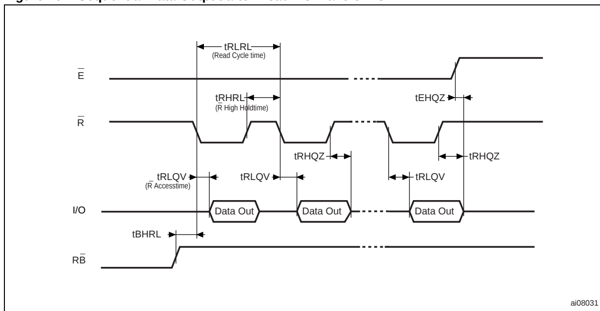
Figure 26. Sequential Data Output after Read AC Waveforms
