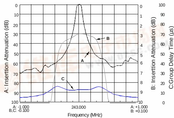
HF-363A 243 MHz
