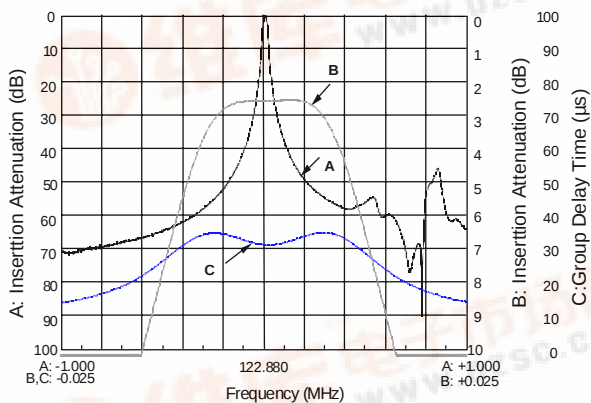
HF-362A 122.88 MHz
