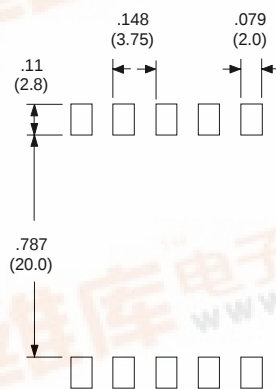
Suggested Solder Pad Layout
