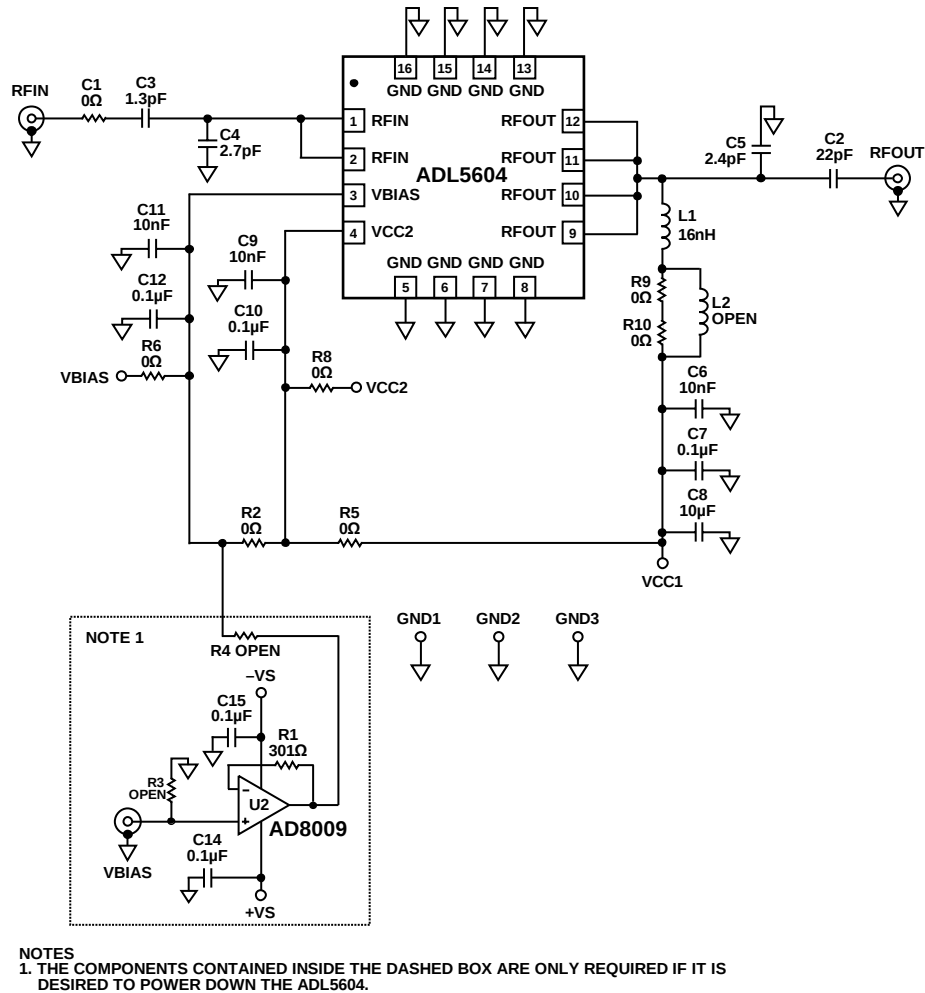
Figure 35. Basic Connections
