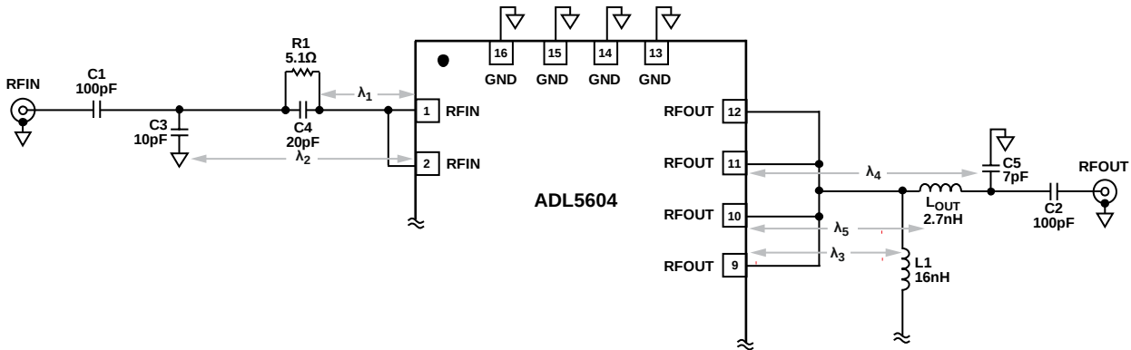
Figure 36. ADL5604 Match Parameters, 748 MHz
