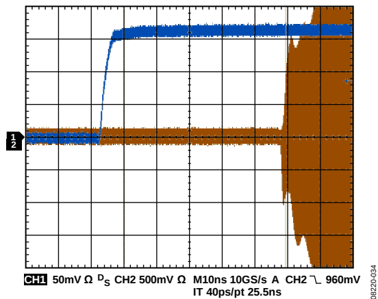
Figure 34. Turn -On Time, 50% of Control Pulse to 50% of RF Burst
