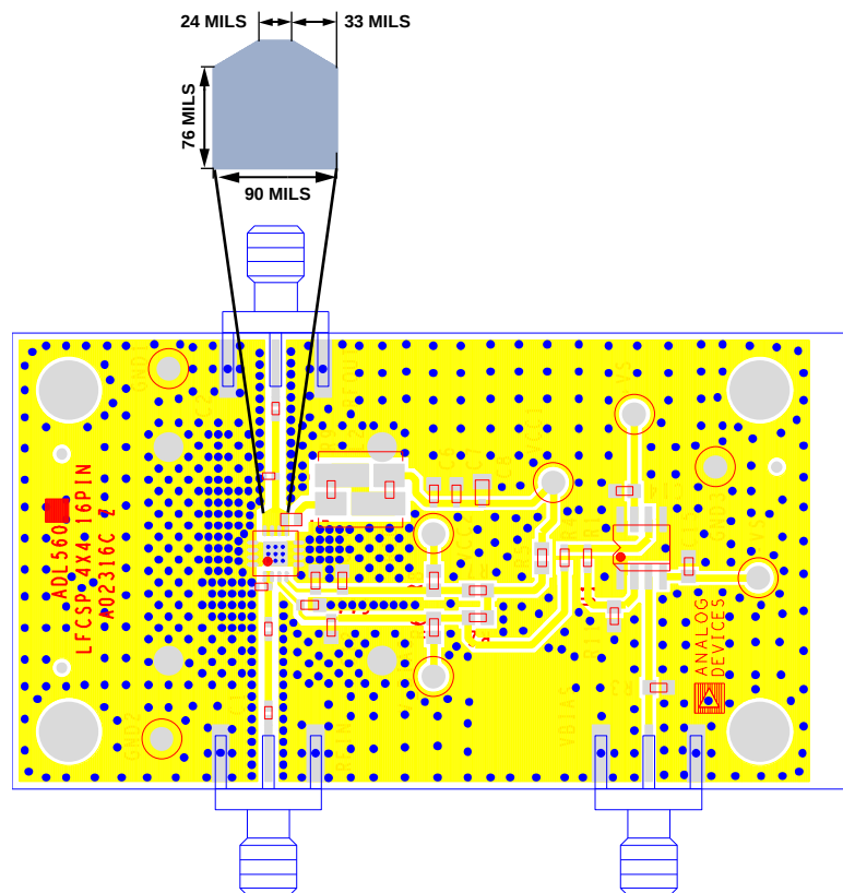
Figure 46. Evaluation Board Layout, Output Pad
