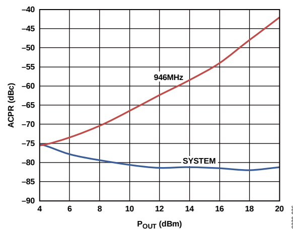
Figure 26. ACPR vs. P_{OUT} , 3GPP 3.5 TM1-64 at 946 MHz
