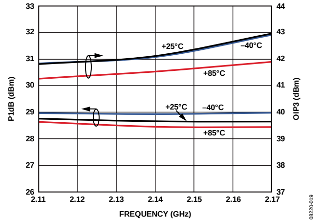
Figure 19. OIP3 at P_{OUT}=14 dBm/Tone and P1dB vs. Frequency and Temperature
