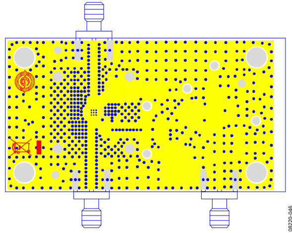
Figure 45. Evaluation Board Layout, Bottom Side
