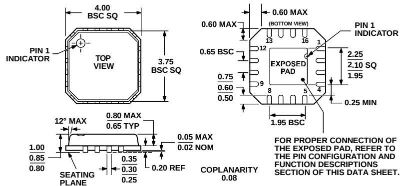
Figure 47. 16-Lead Lead Frame Chip Scale Package [LFCSP_VQ] 4 mm x 4 mm Body, Very Thin Quad (CP-16-4)
