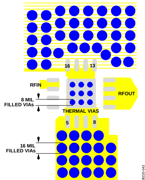
Figure 42. Recommended Land Pattern
