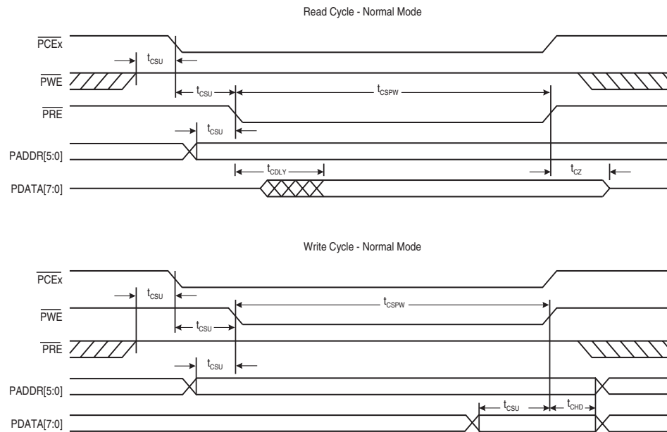
Figure 5 - Normal Reading and Writing From a Control Register
