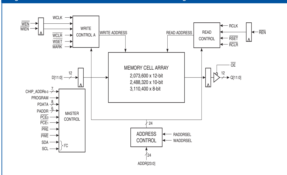
Figure 3. Random Access Mode Functional Block Diagram
