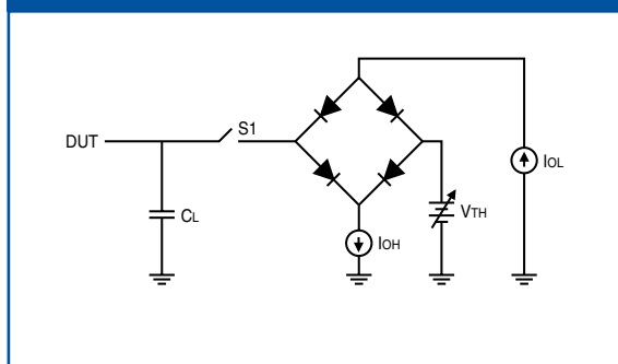
FIGURE A. OUTPUT LOADING CIRCUIT
