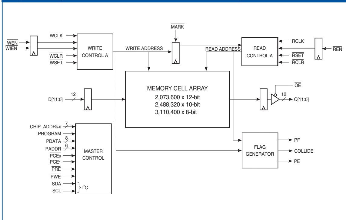
Figure 2. Single Channel FIFO Mode Functional Block Diagram
