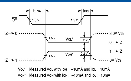
FIGURE B. THRESHOLD LEVELS
