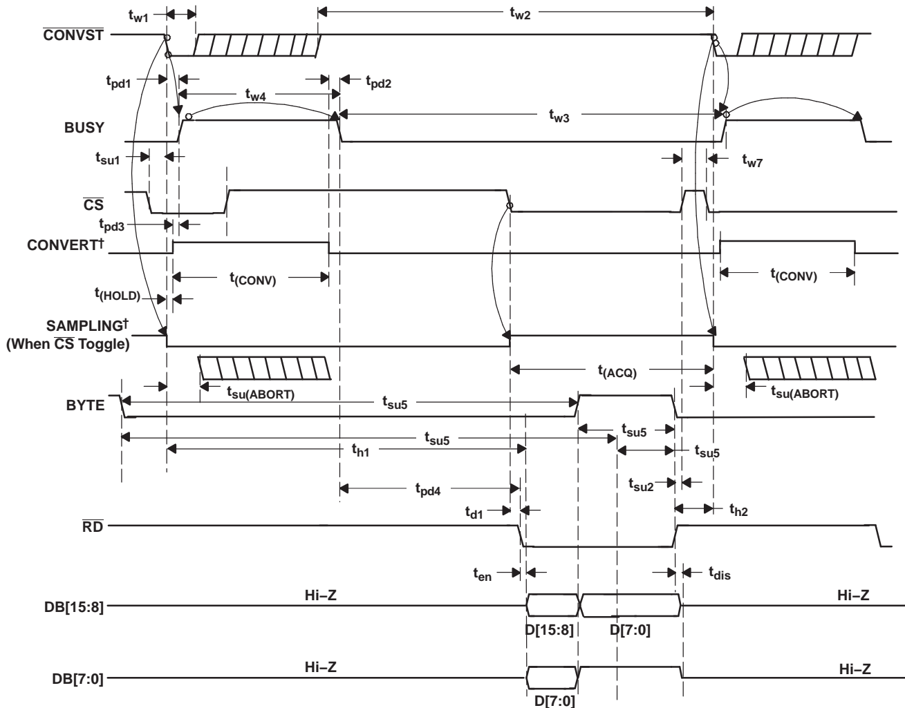
Figure 32. Timing for Conversion and Acquisition Cycles With CS and RD Toggling
