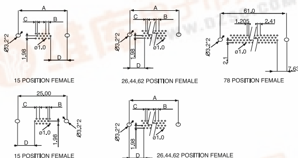
P.C.BOARD LAYOUT PATTERN
