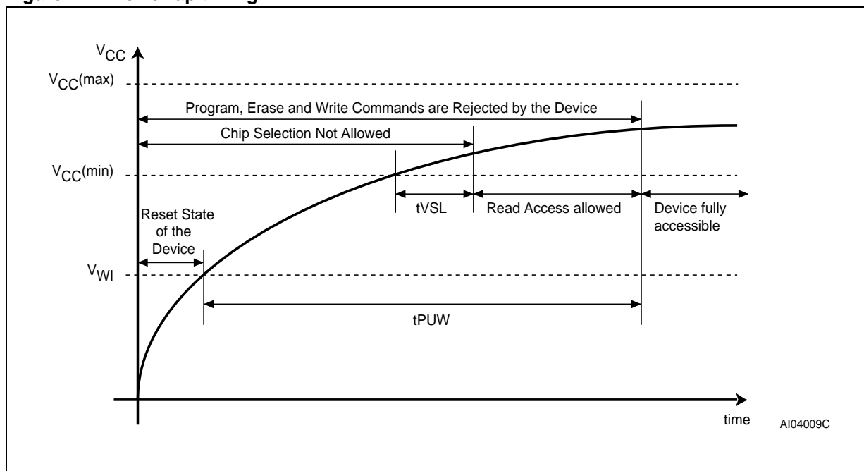
Figure 24. Power-up timing
