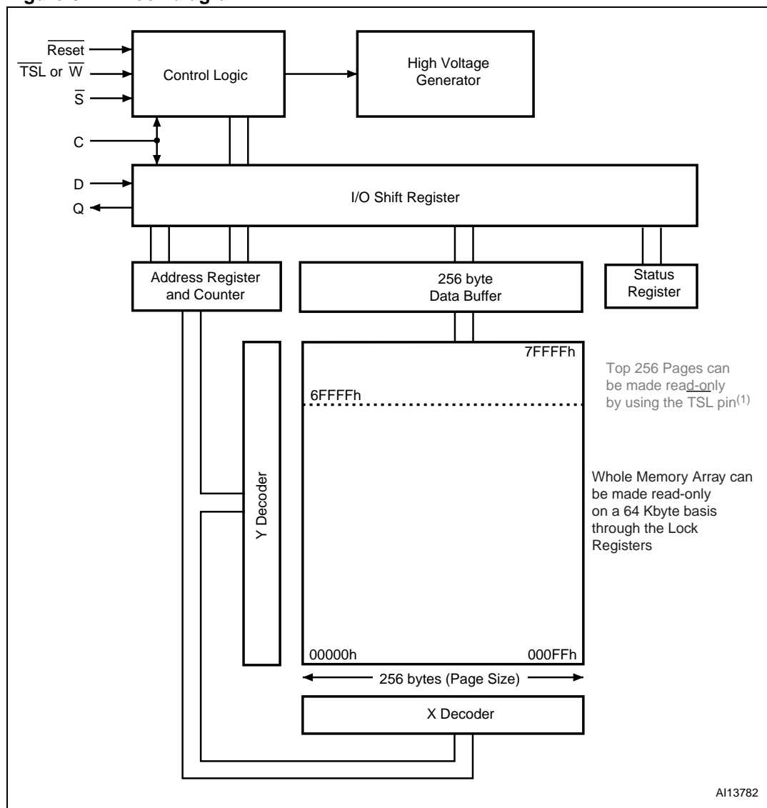
Figure 6. Block diagram
