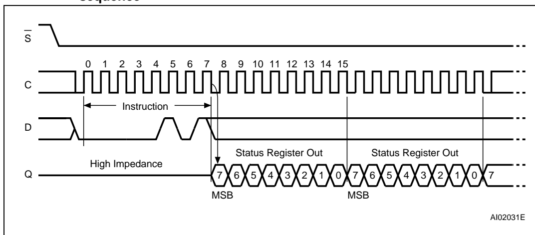
Figure 10. Read Status Register (RDSR) instruction sequence and Data-out sequence
