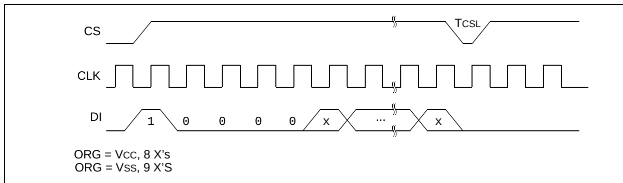
FIGURE 3-4: EWDS
