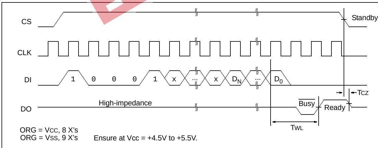
FIGURE 3-6: WRAL
