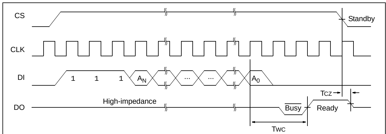
FIGURE 3-7: ERASE
