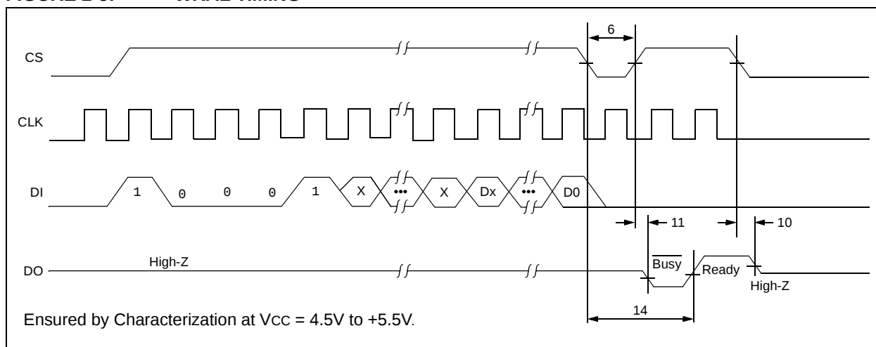
FIGURE 2-5: WRAL TIMING
