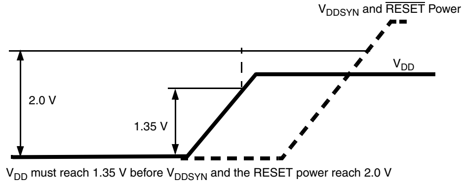
Figure 2. Power-Up Sequence (V RC33 Grounded)
