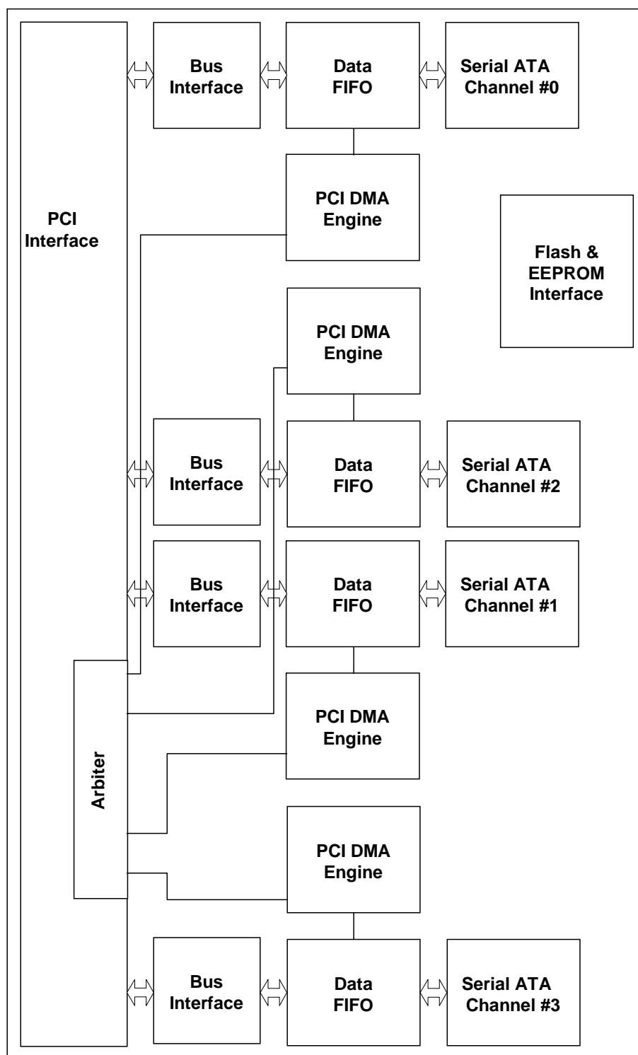
Figure 7. Sil3114 Block Diagram
