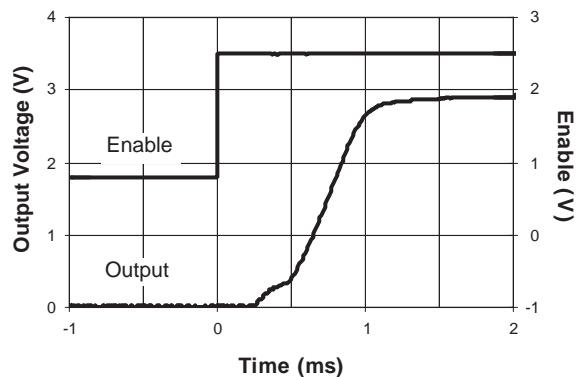
Turn-On with 10mA Load
