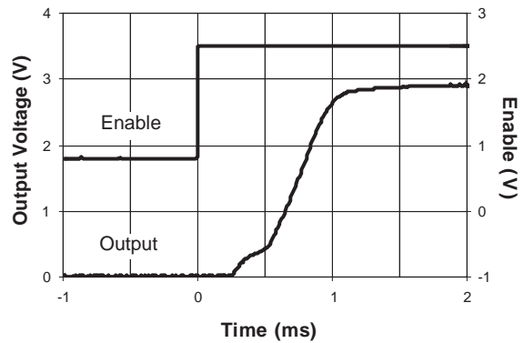
Turn-On with 1mA Load
