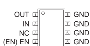
AAT3221 SC70JW-8 (Top View)
